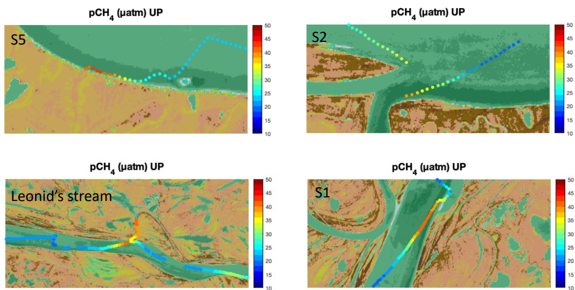
Figure S3 – Closer view to the measured surface p\text{CH}_4 in key sites and at Leonid's stream, where larger methane concentrations were observed compared to the surrounding areas.
