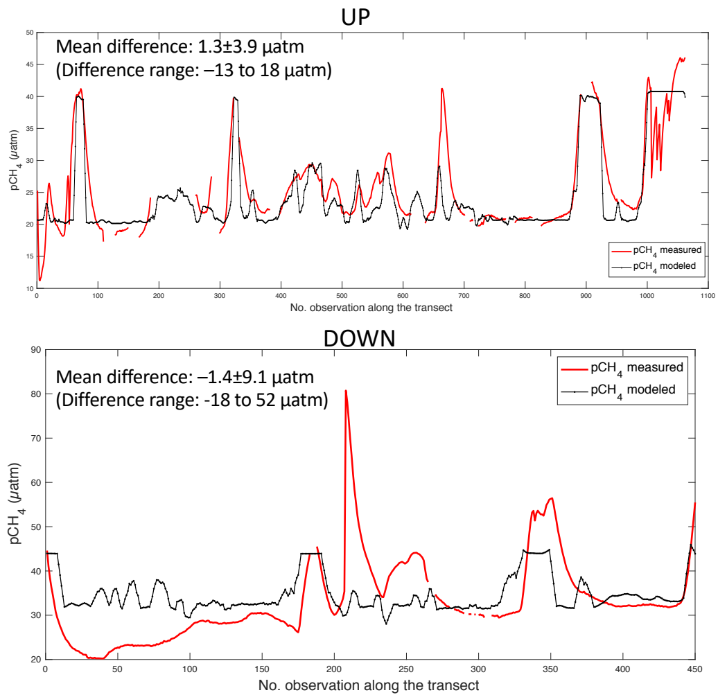
Figure S7 – Comparison between modeled pCH_4 from random forest regression and measured pCH_4 along the UP (top) and DOWN (bottom) transects.
