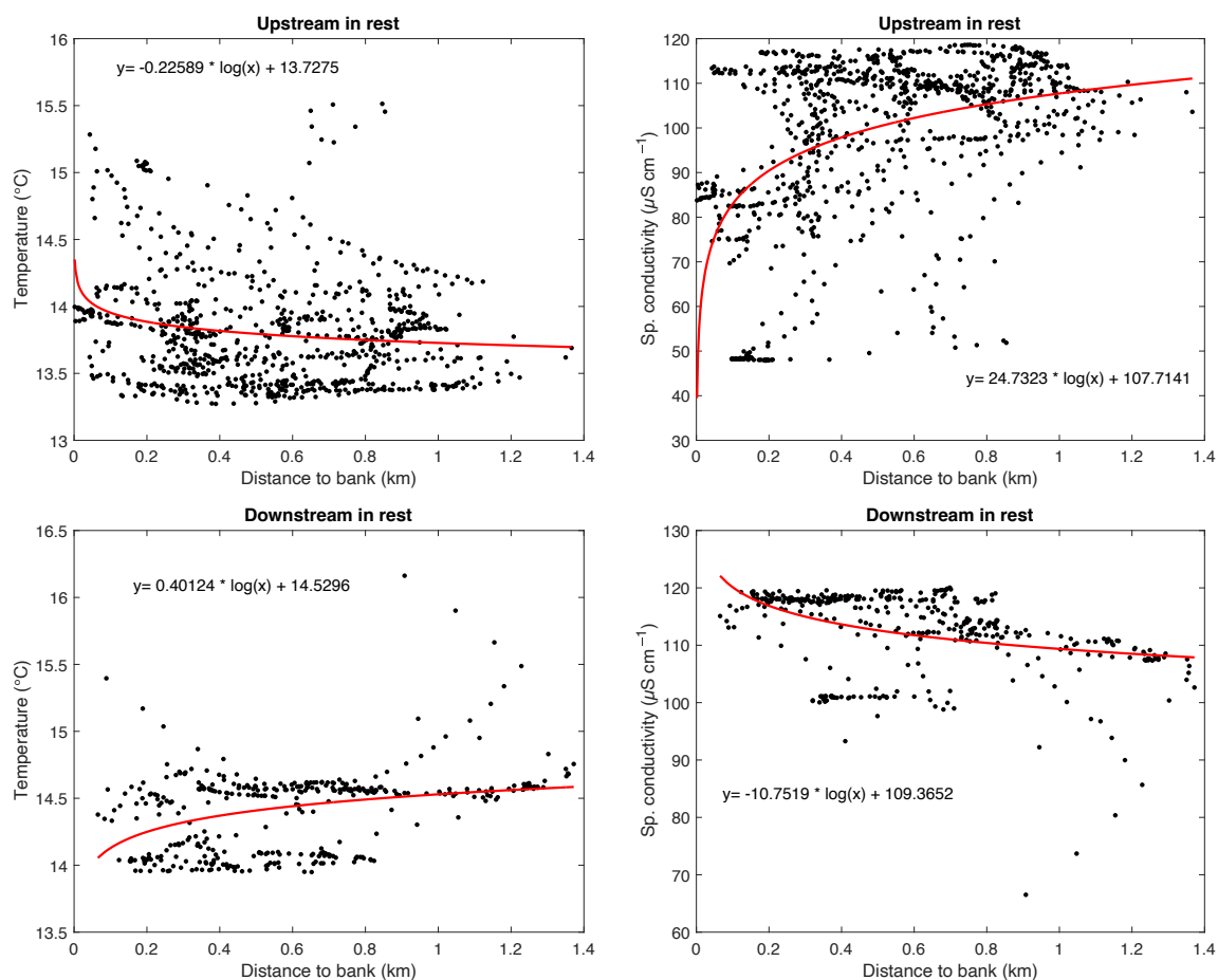
Figure S5 – Linear correlation analysis between the conservative properties temperature and specific conductivity against the distance to bank z during the UP and DOWN transects for data in other sites the transect.
