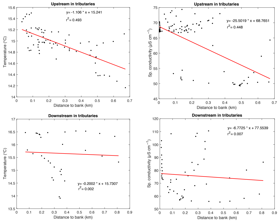
Figure S4 – Linear correlation analysis between the conservative properties temperature and specific conductivity against the distance to bank z during the UP and DOWN transects for key sites.
