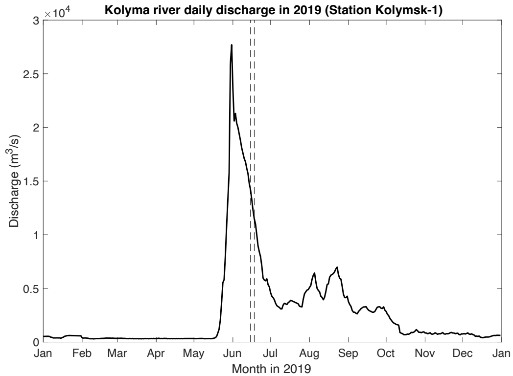
Figure S1 - Water discharge curve in Kolyma River in 2019 , data from Arctic Great Rivers Observatory (Shiklomanov et al., 2020). Discharge curve during freshet period from 20 May ( 840 \text{ m}^3 \text{ s}^{-1} ) to 10 July ( 3090 \text{ m}^3 \text{ s}^{-1} ). Peak of the freshet: 31 May ( 27,700 \text{ m}^3 \text{ s}^{-1} ). Vertical dashed lines indicate the sampling dates during the upstream transect (left line, 15-16 June 2019) and the downstream transect (16-17 June 2019).
