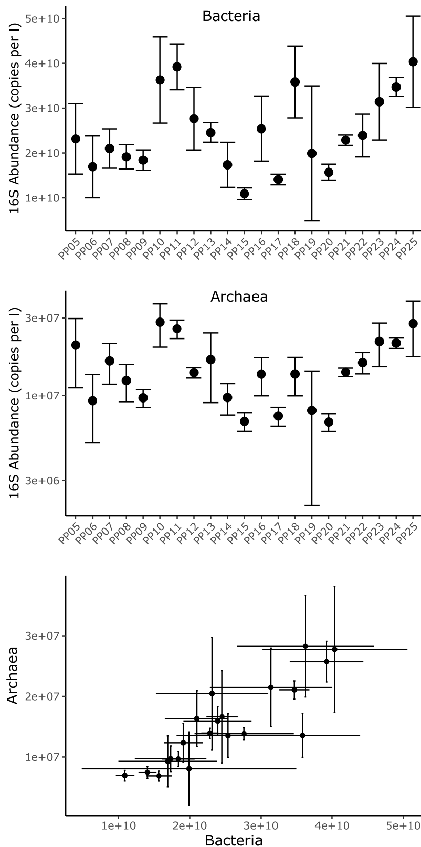
Figure S8 – qPCR graph showing the 16S abundance of bacteria (top) and archaea (middle) in samples from Kolyma River. Despite bacteria is three orders of magnitude more abundant than archaea, there is a positive linear correlation between them (bottom).
