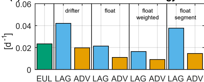
(c) metbio003d host bin -- climatology subtrahend
