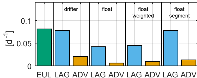
(b) metbio010d host bin -- smoothed subtrahend
