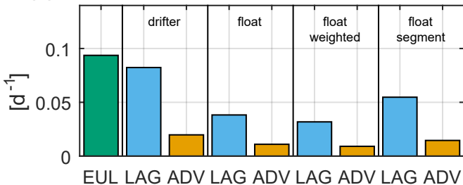
(a) metbio003d host bin -- smoothed subtrahend
