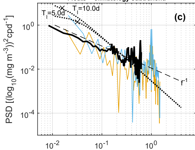
Floats -- climatology subtrahend
