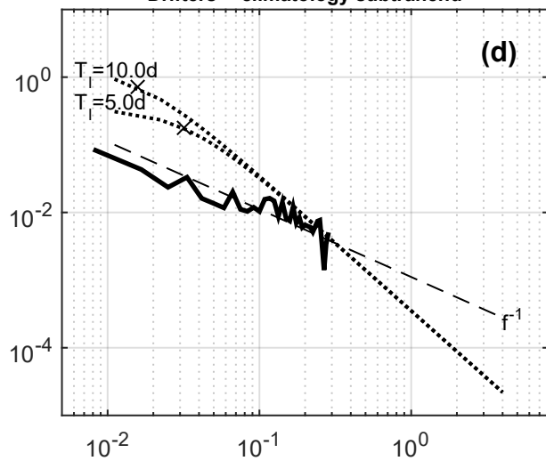
Drifters -- climatology subtrahend
