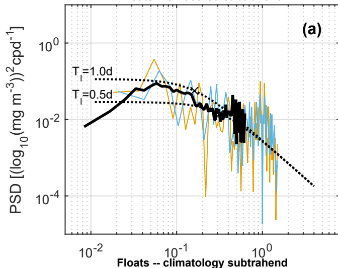
Floats -- smoothed subtrahend
