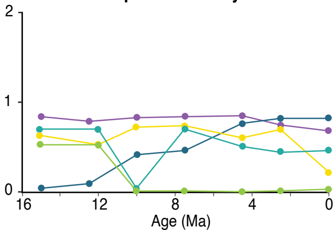
Simpson Diversity Index
