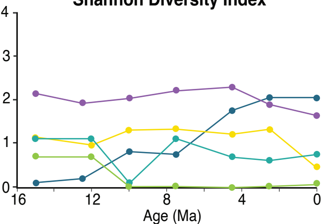
Shannon Diversity Index
