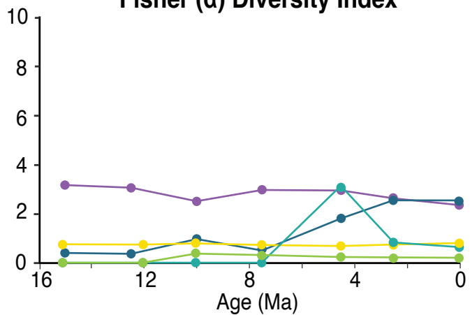
Fisher ( \alpha ) Diversity Index
