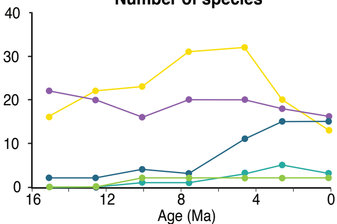
Number of species
