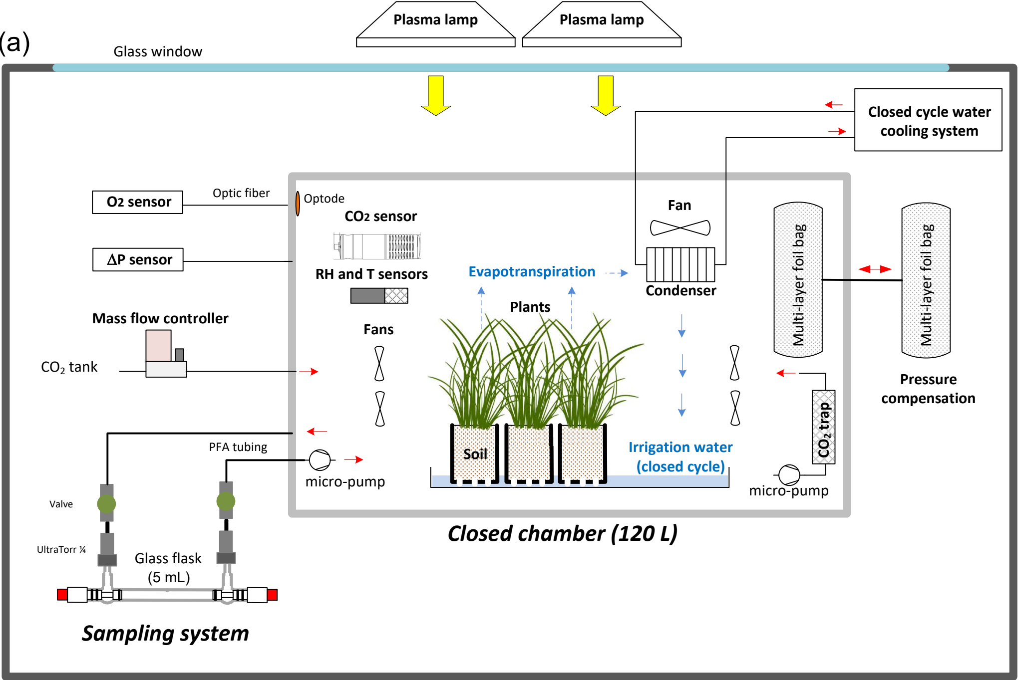
Growth chamber
