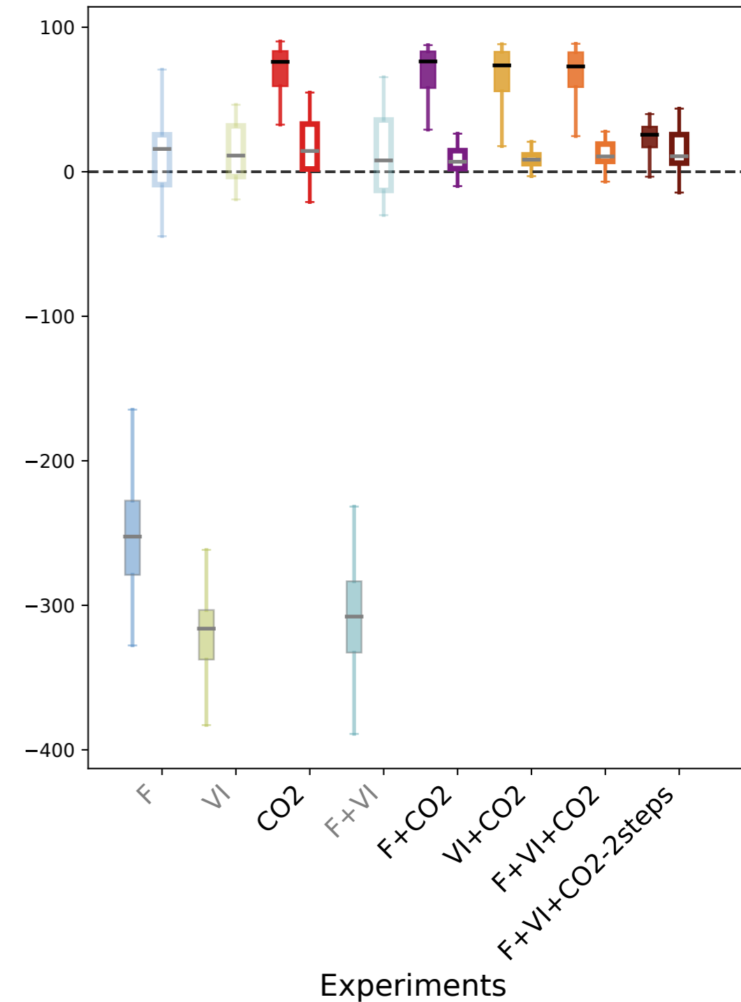
(c) CO2atm
