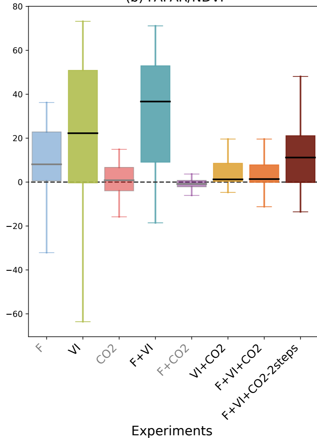
(b) FAPAR/NDVI
