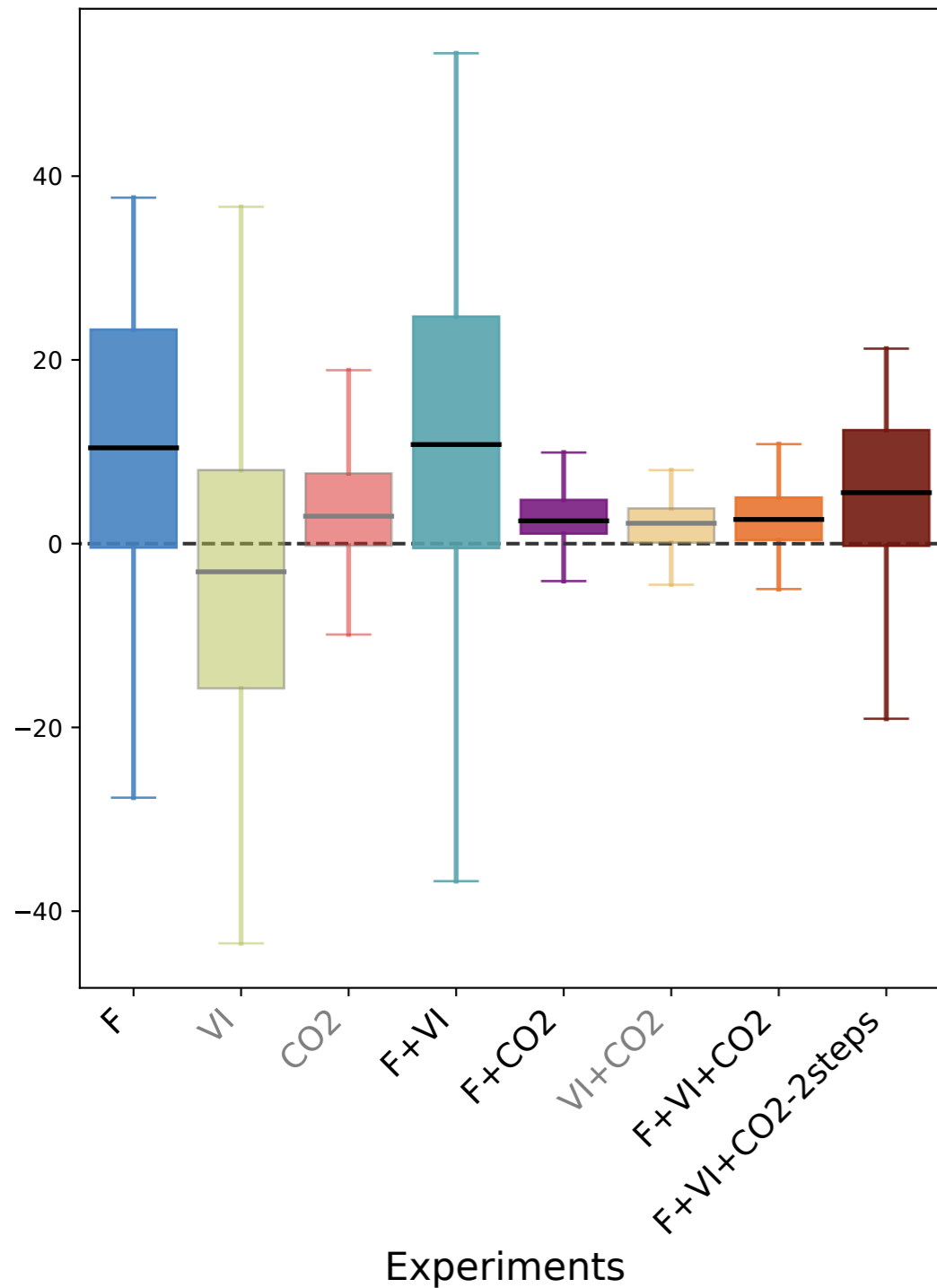
(a) NEE
