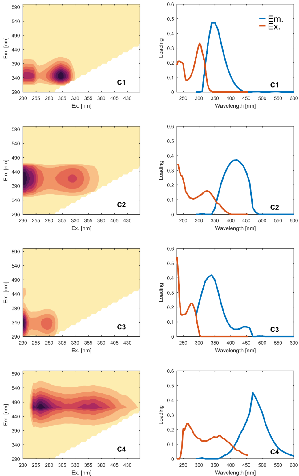
Supplementary Fig S1. FDOM components (C1-C4) derived from the PARAFAC analysis. Left column: EEMs of each component. Right column: corresponding excitation and emission loadings.
