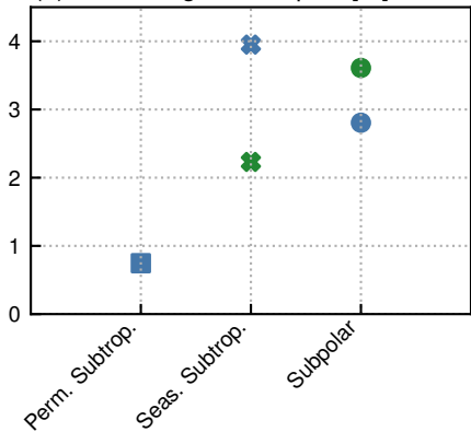
(b) Chl-a global surplus [%]
