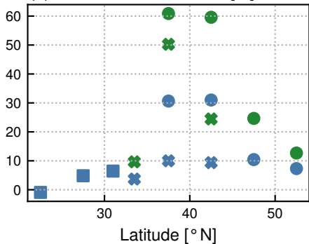
(a) Local Excess Chl-a [%]
