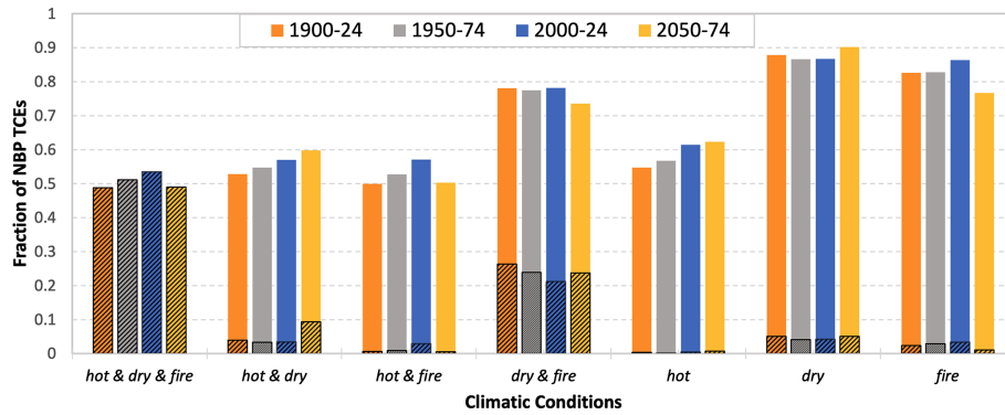
Figure 5. Fractional distribution of carbon cycle time-continuous extremes (TCEs) driven by compound climate drivers at a lag of 1 month. The unhatched and hatched bars represent the mutually inclusive and exclusive compound and individual climate drivers, respectively. The exclusive climate drivers are always less than or equal to mutually inclusive drivers. The different colored bar represents following periods: 1900–1924, 1950–1974, 2000–2024, and 2050–2074 (from left to right bar). Most carbon cycle extremes are driven by the interactive effect of climate drivers.
