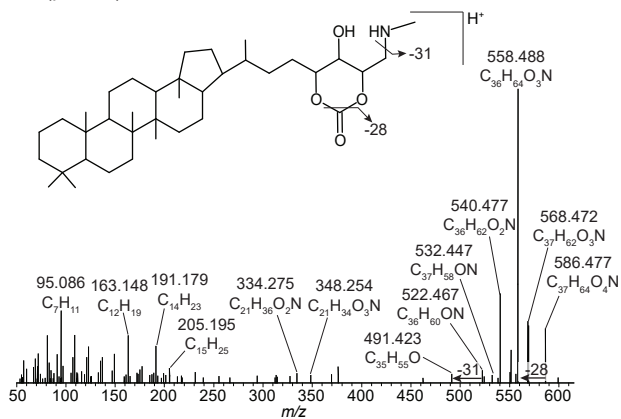
(e) MS 2 of m/z 618.473, [M+H] + of \Delta^{11} -ethanolamine-BHhexol (peak i)
