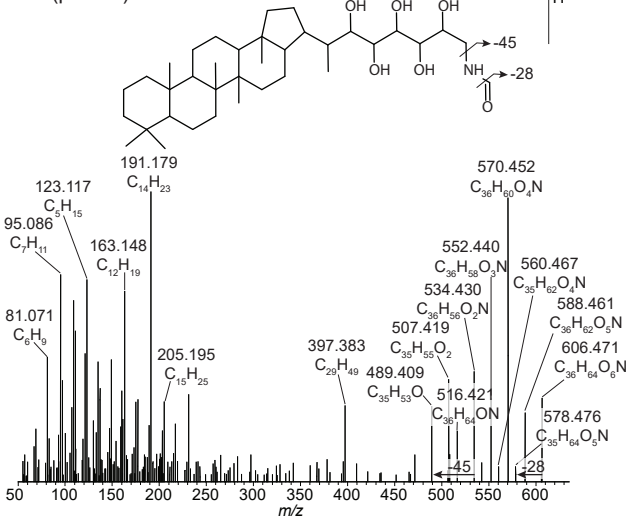
(f) MS 2 of m/z 606.4, [M+H] + of N-formylated aminopentol (peak o)
