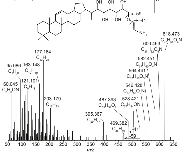
(e) MS 2 of m/z 618.473, [M+H] + of \Delta^{11} -ethanolamine-BHhexol (peak i)
