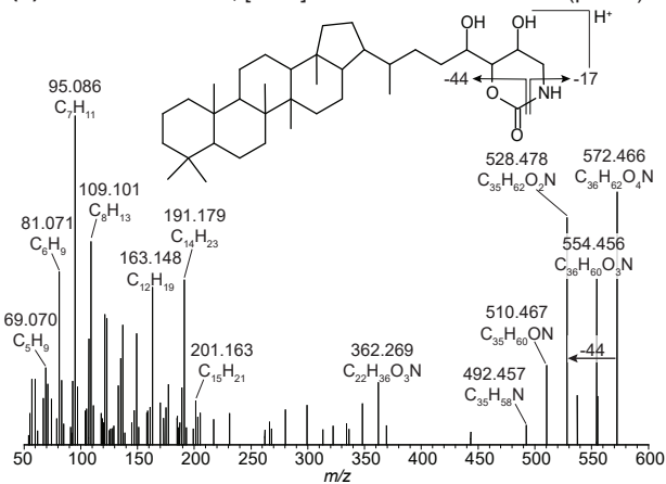
(f) MS 2 of m/z 606.4, [M+H] + of N-formylated aminopentol (peak o)
