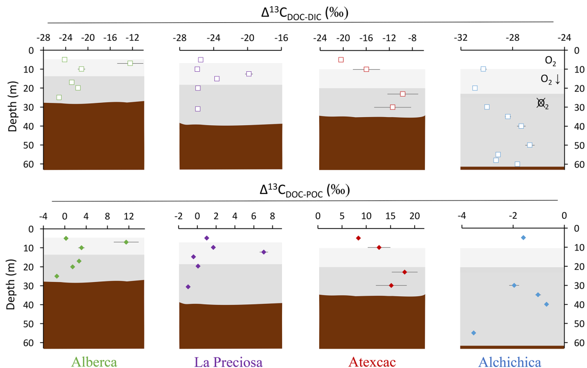
Figure 4. Vertical profiles of the difference in \delta^{13}C values of DOC and DIC (top) and of DOC and POC (bottom) throughout the water columns of the four lakes (all expressed as \Delta^{13}C in ‰ vs. VPDB). POC and DIC data used in these calculations are from Havas et al. (2023a). In Alchichica, \delta^{13}C_{DOC} was not measured at 5 m, and its value at 10 m was used in this calculation of \Delta^{13}C_{DOC-POC} . The white, gray, and dark-gray shading are as in Fig. 2. The brown shading symbolizes the presence of sediment at the bottom of the water columns.
