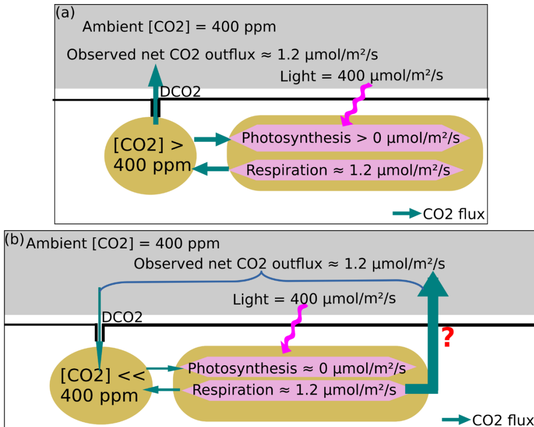
Figure S15: The schematic diagram of the CO 2 diffusion pathways. (a): the pathway in the data-driven model, which makes it impossible to fit a strongly negative net C flux. (b): The pathway that allows a simulation of strongly negative net C flux. Please note that the figure only shows CO 2 fluxes. Contrary to vascular plants, CO 2 and water exchange are not coupled in lichens and mosses, due to lack of stomata. The model thus calculates water fluxes independently based on the surface energy balance.
