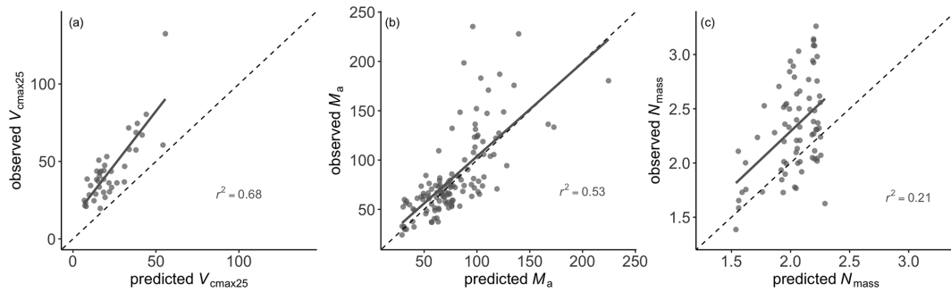
Figure 6. Optimality-based predictions versus observations of leaf traits at the site level. Grey lines are ordinary least-squares regressions. The black dashed line is the 1 : 1 line.
