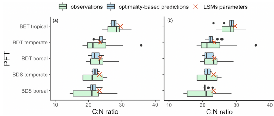
Figure 7. Comparison of observed and predicted C : N ratios with target values in LSMs. The blue boxes represent predicted C : N ratios using observed C_{mass} (a) and using constant mean C_{mass} (b). The green boxes represent observed C : N ratios. Red crosses show target values in LSMs (adopted from CLM4).
