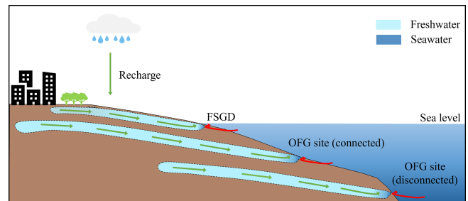
Figure 1. Schematic representation of known pathways for the transport and storage of fresh and freshened groundwater between terrestrial and marine realms. Areas surrounded by dashed lines indicate groundwater reservoirs, whereas arrows represent freshwater (green) and seawater (red) fluxes. Based on Bratton et al. (2010) and Weymer et al. (2020).
