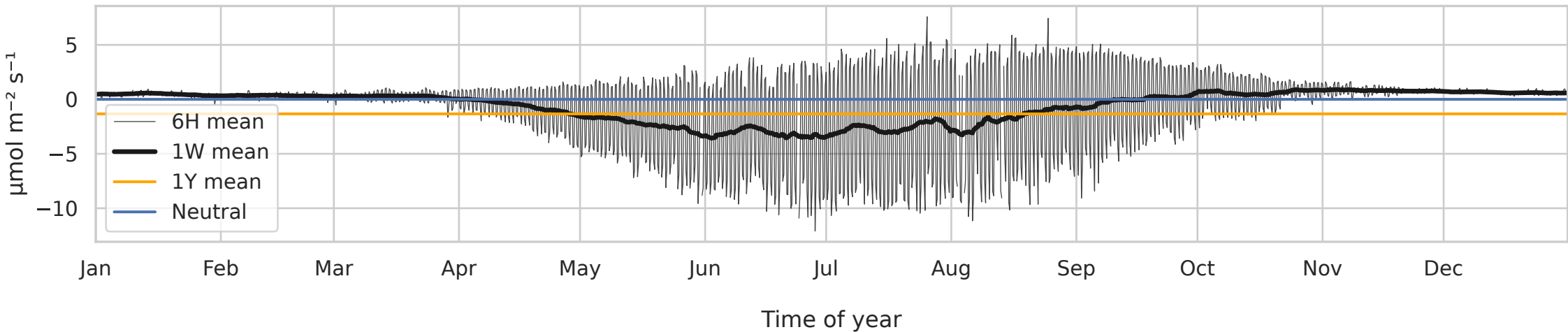
Multi-year means of the measured net ecosystem CO 2 exchange
