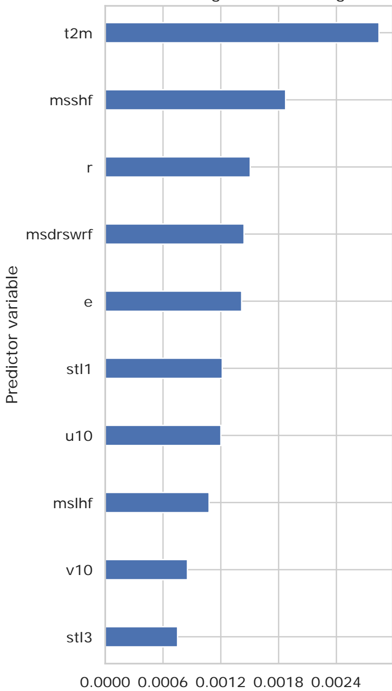
(a) mean(|SHAP|) over models, grid cells and lags
