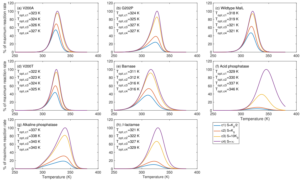
Figure S1. Substrate availability strongly affects the temperature sensitivity of the enzymatic reaction rates, as shown for the 8 example enzymes that are not shown in Figure 3 of the main text.
