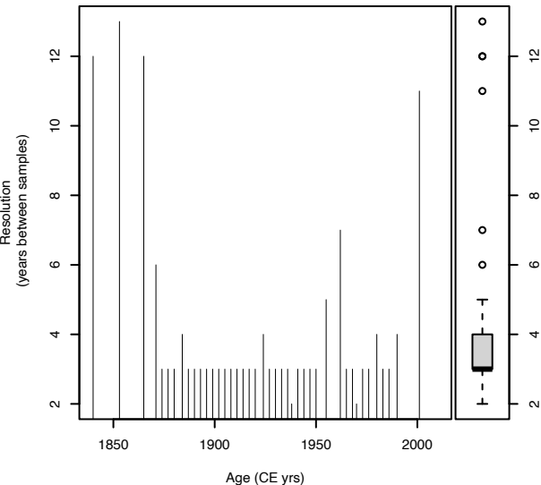
(a) AVG-pollen
