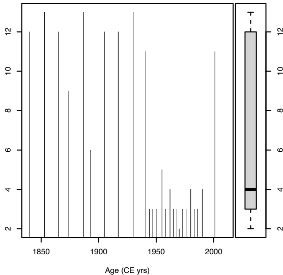
(b) AVG-diatoms
