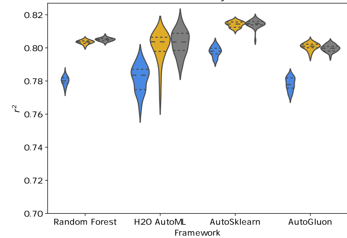
Seasonality
