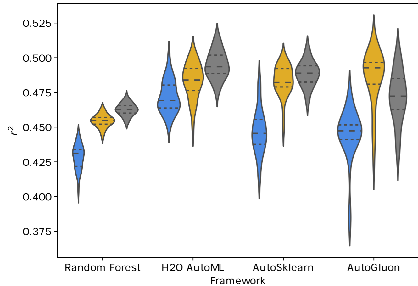
Seasonality
