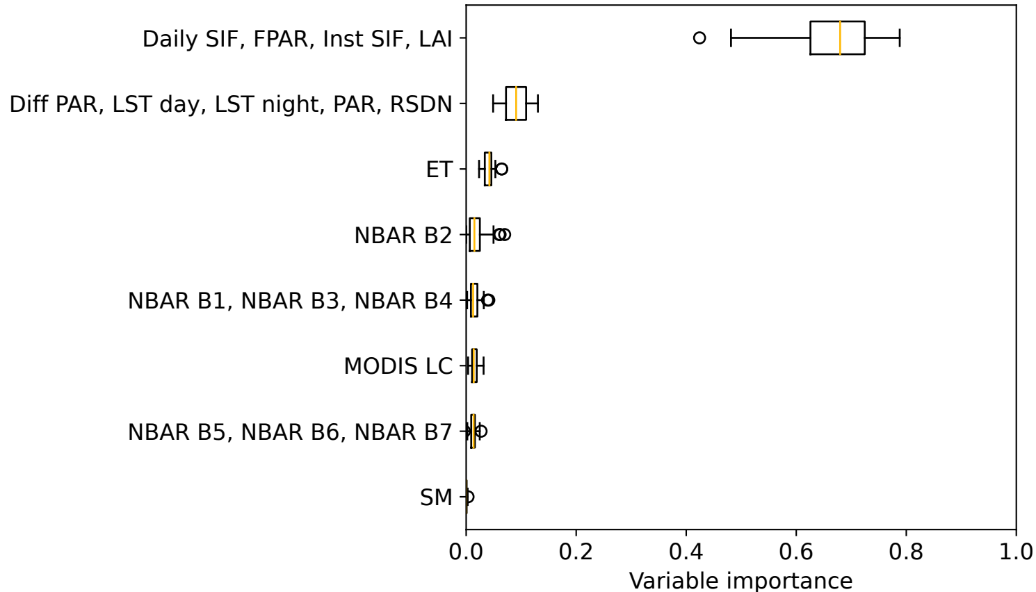
AutoSklearn-RS
