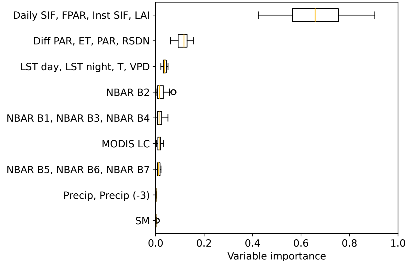
AutoSklearn-RS meteo
