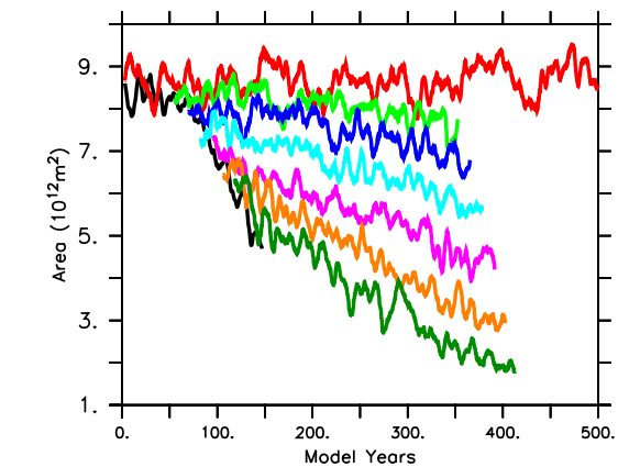
(f) Average Antarctic sea ice area
