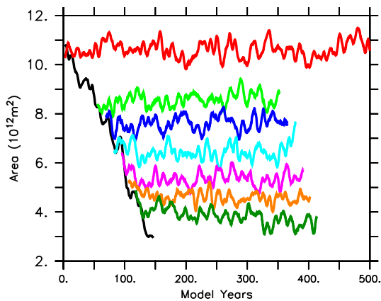
(e) Average Arctic sea ice area
