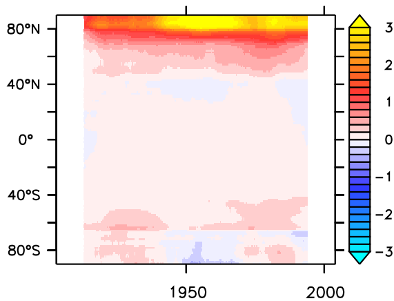
(h) UKESM ZEC750
