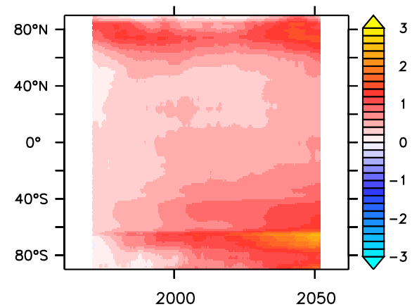
(i) UKESM ZEC2000
