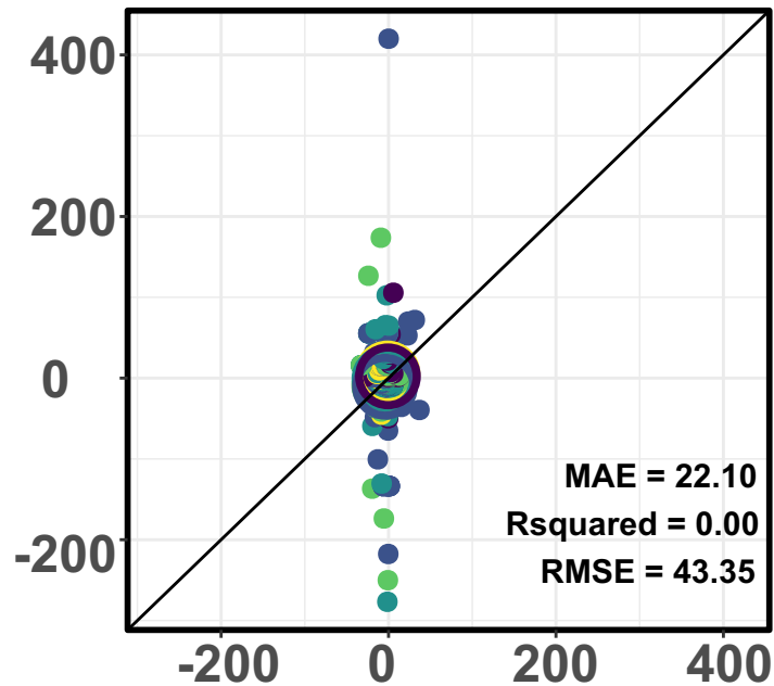
N 2 O flux μg N m -2 d -1
