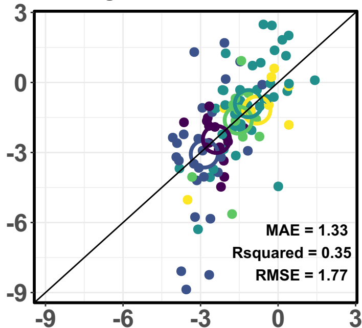
NEE g C m -2 d -1
