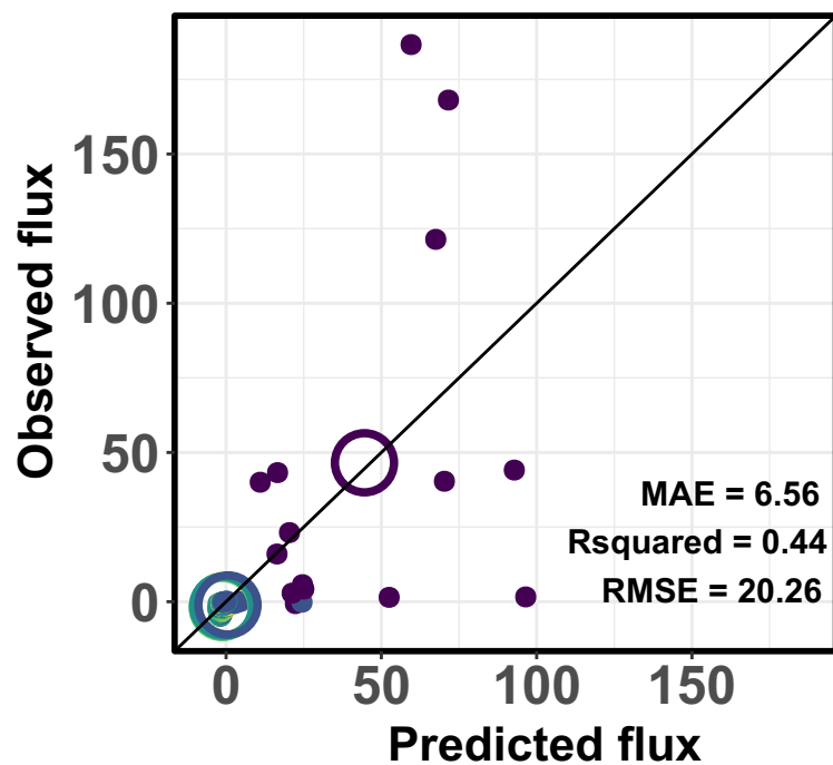
CH 4 flux mg C m -2 d -1
