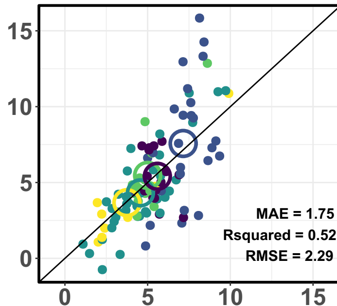
GPP g C m -2 d -1
