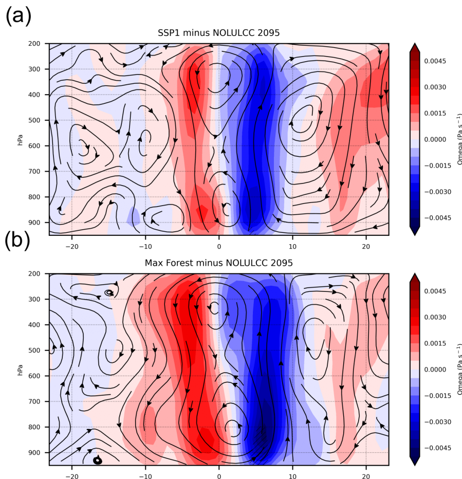
Figure 9. Differences in the Hadley circulation between scenarios at the end of the 21st century. Contour data are vertical velocity ( \omega ); streamlines are the resultant vectors of \omega \times 1000 and meridional wind. Data are averaged over tropical latitudes.
