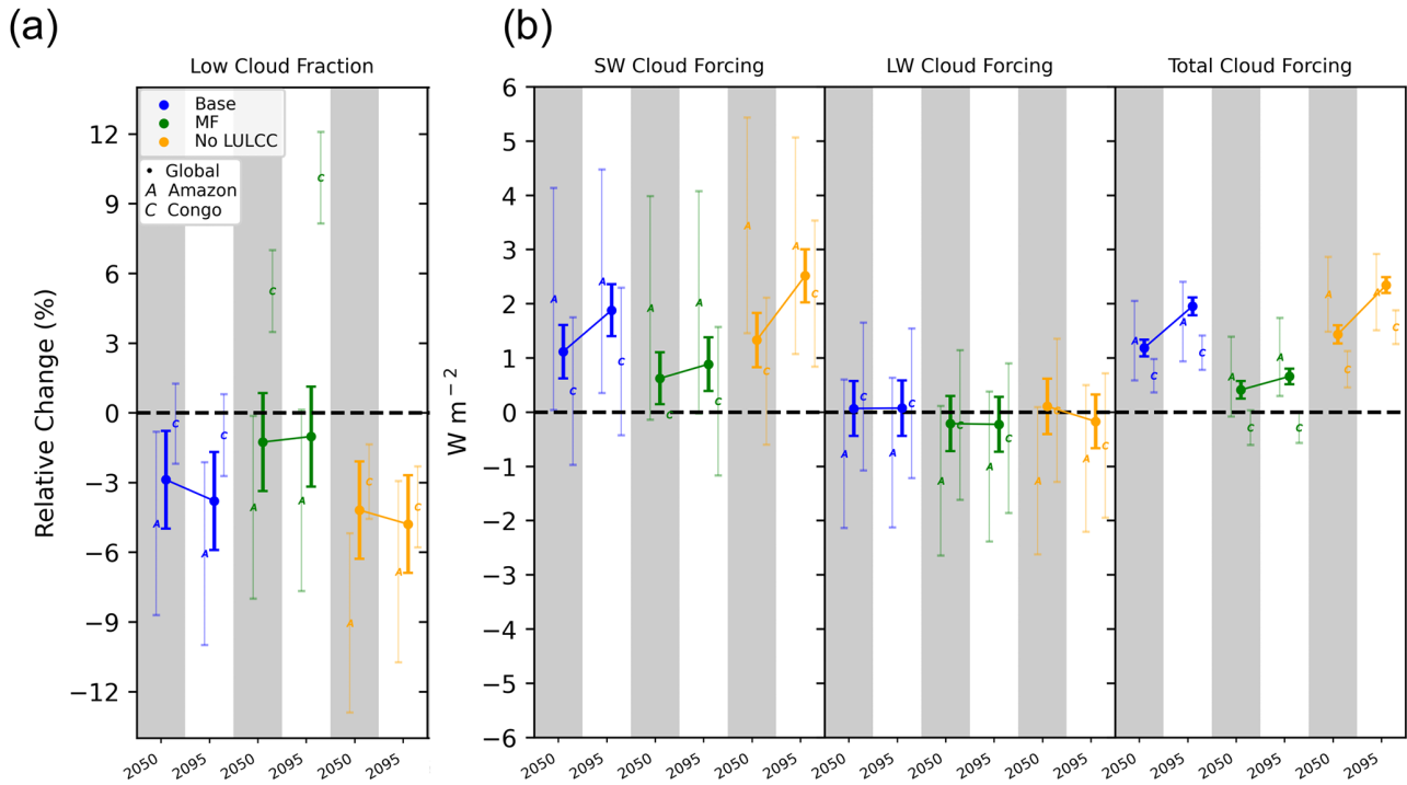
Figure 7. As Fig. 2b but showing differences in cloud cover integrated between 1200–700 hPa (a) and differences in clean-sky shortwave cloud radiative forcing, clean-sky longwave cloud radiative forcing, and total clean-sky cloud radiative forcing (b).
