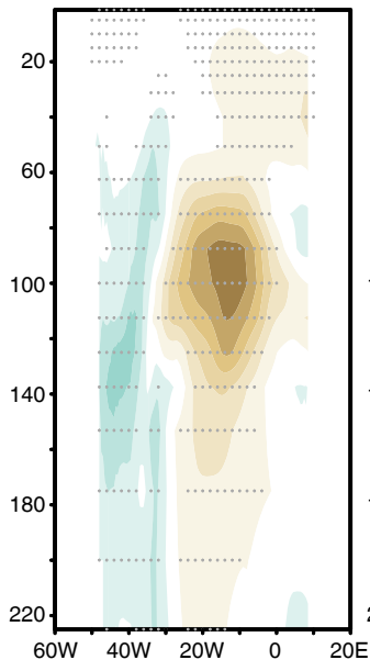
(a) NorESM1-CTL
