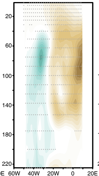
(c) NorESM2-LM
