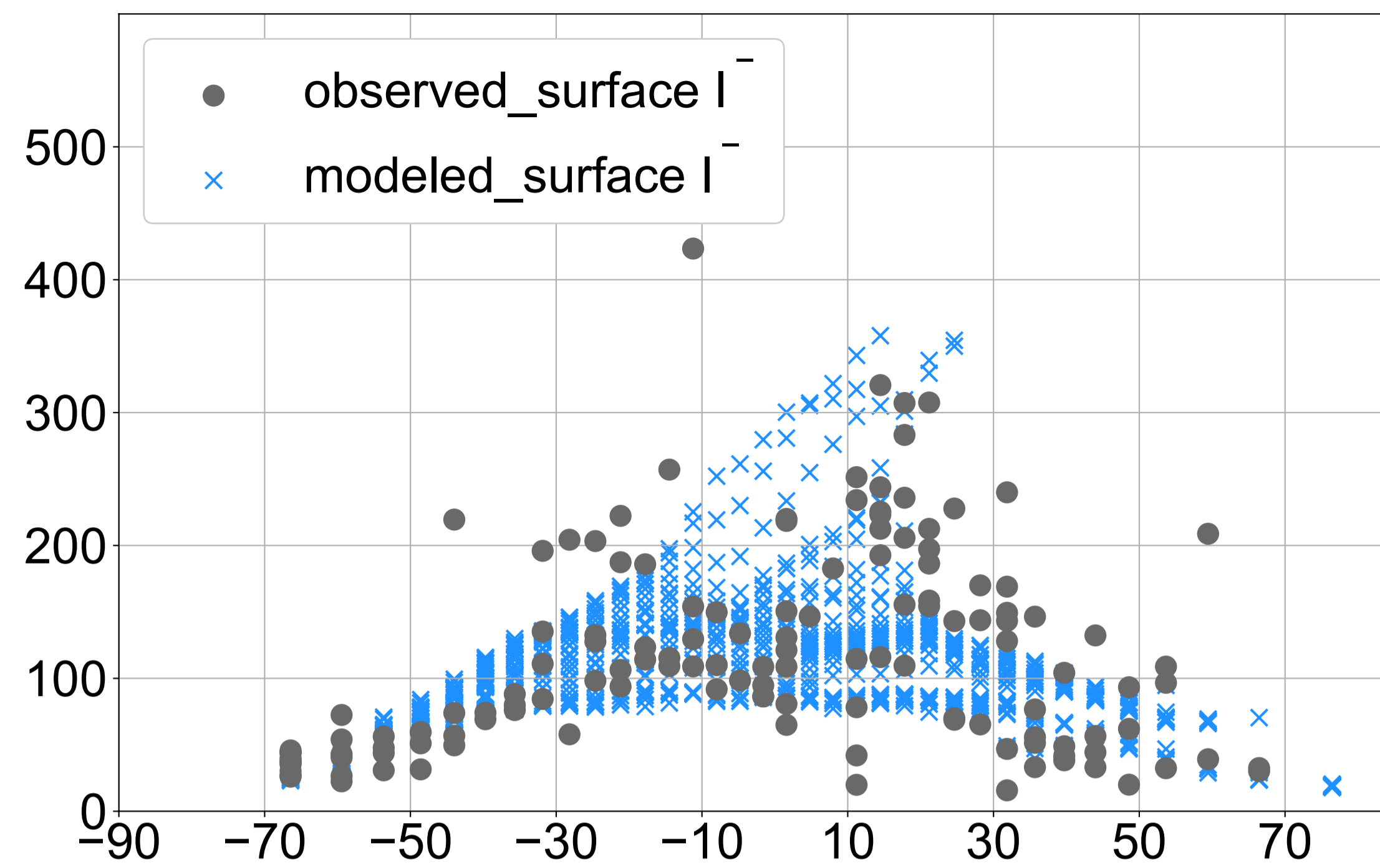
WOA-forced [O 2 ]
