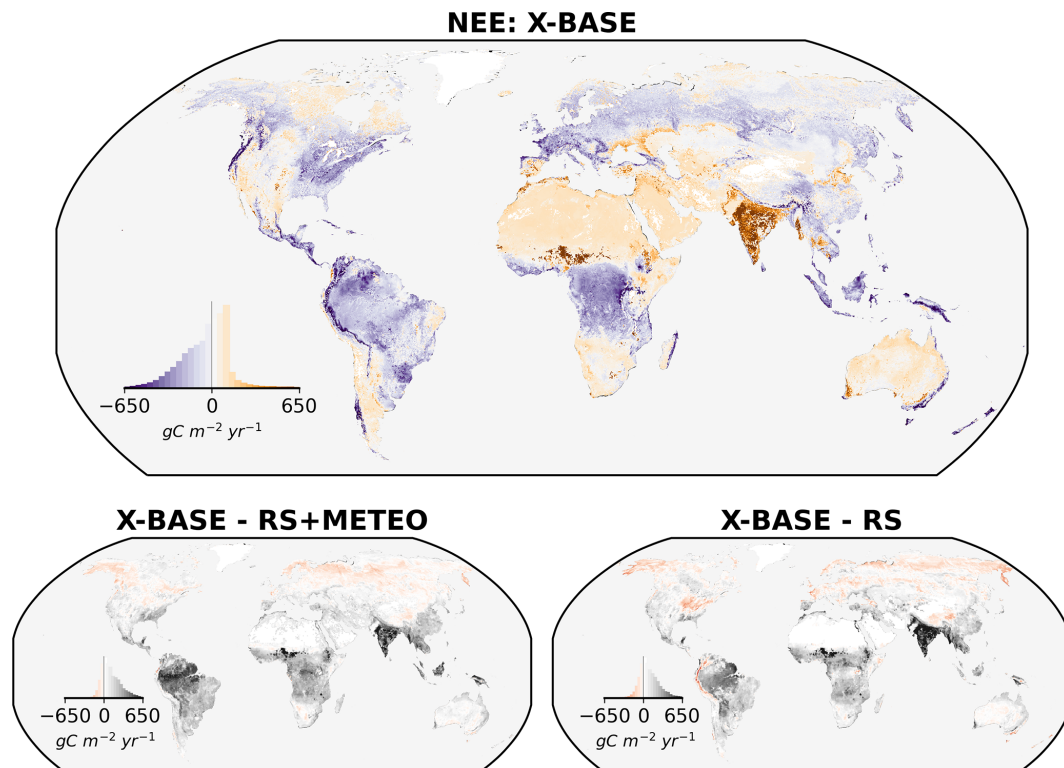
Figure 4. Comparison of annually integrated NEE from X-BASE, RS + METEO with ERA5 forcing, and RS averaged over the period 2001–2020. The difference maps show the difference of the averages over 2001–2020.
