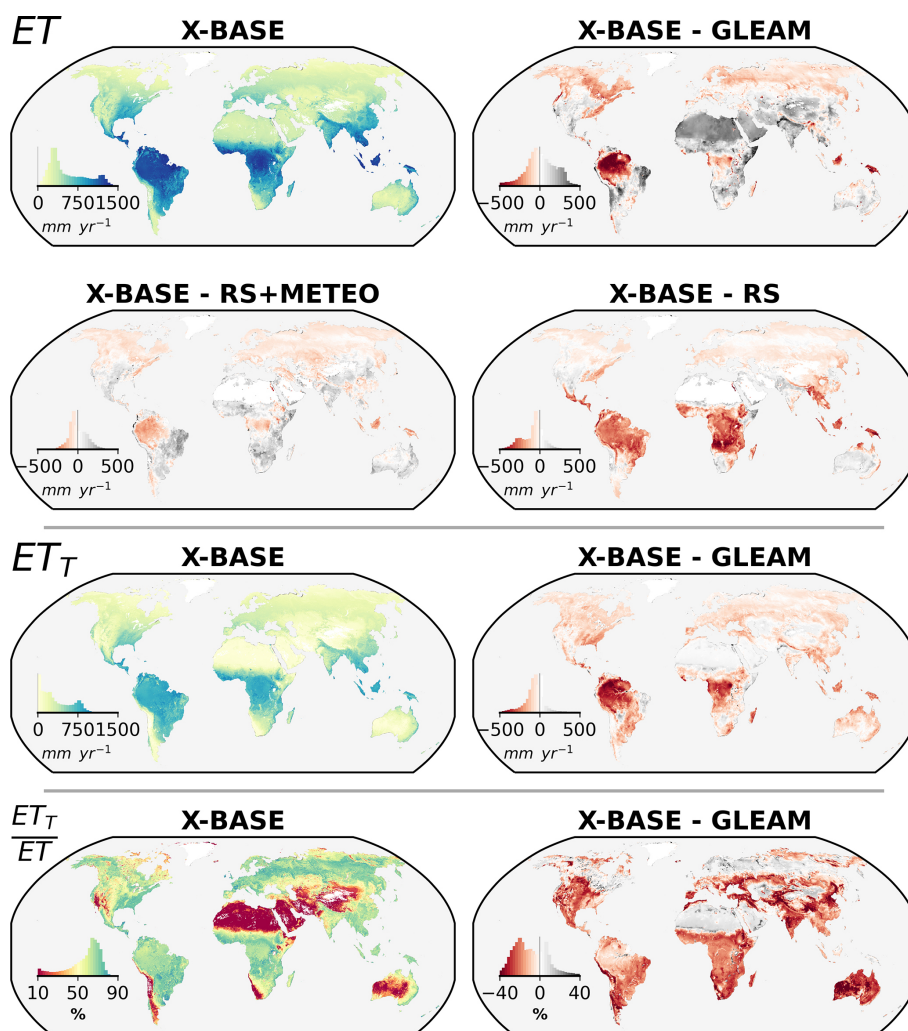
Figure 8. Comparison of evaporative flux estimates ET , ET_T , and ET_T/ET from X-BASE and its difference with RS, RS + METEO, and GLEAM. ET_T is compared in the case of GLEAM but is unavailable in the previous FLUXCOM ensembles.
