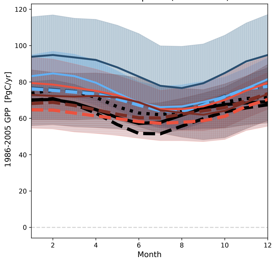
Southern Hemisphere (20°S - 90°S)
