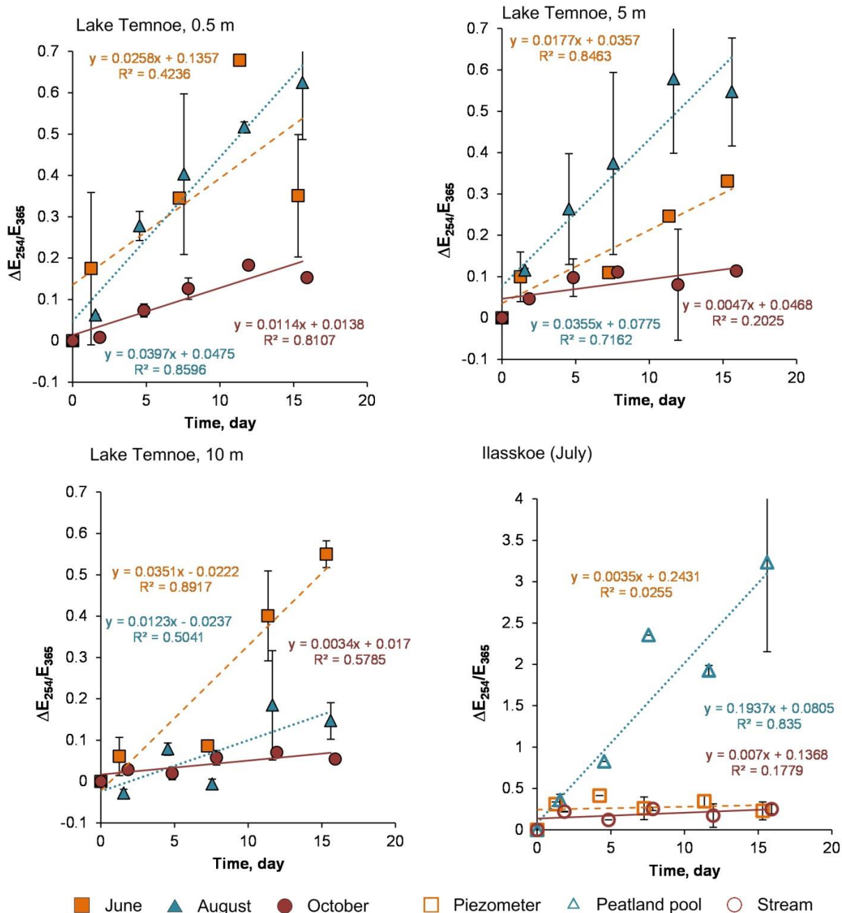
Fig. S11. The change of optical ratios ( E_{254}/E_{365} ) over time in photodegradation experiments. Lake Temnoe 0.5 m (A), 5 m (B) and 10 m (C) in June (squares), August (triangles) and October (circles). Ilasskoe continuum in July (D) includes piezometer (squares), peatland pool Severnoe (triangles) and stream Chernyi (circles)
