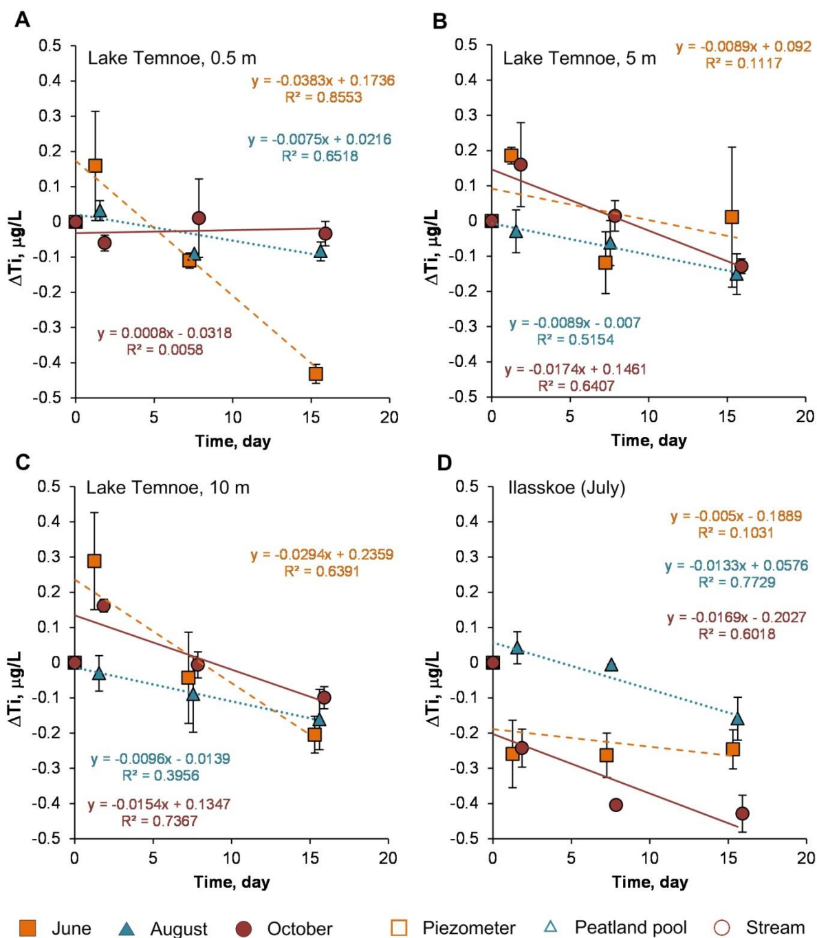
Fig. S13. Change in Ti concentration (relative to the control) over time in photodegradation experiments. The error bars are 1 s.d. of duplicates. Lake Temnoe 0.5 m (A), 5 m (B) and 10 m
