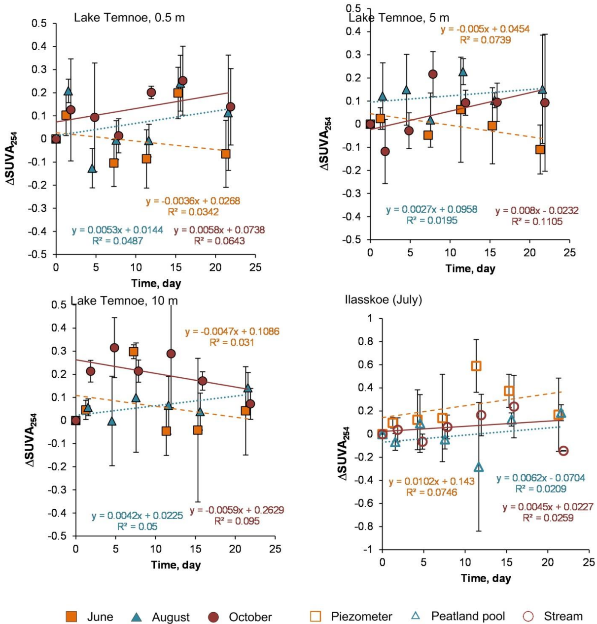
Fig. S2. The change of SUVA_{254} over time in bio-degradation experiments. The error bars represent 1 s.d. of duplicates. Lake Temnoe 0.5 m (A), 5 m (B) and 10 m (C) in June (squares), August (triangles) and October (circles). Illasskoe continuum in July (D) includes piezometer (open squares), peatland pool Severnoe (open triangles) and stream Chernyi (open circles)
