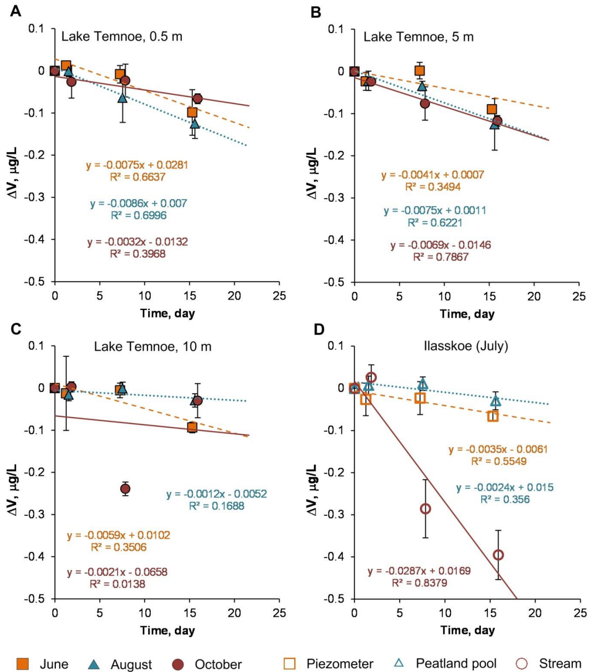
Fig. S7. Change in V concentration (relative to the control) over time in bio-degradation experiments. The error bars are 1 s.d. of duplicates. Lake Temnoe 0.5 m (A), 5 m (B) and 10 m (C) in June (squares), August (triangles) and October (circles). Ilasskoe continuum in July (D) includes piezometer (squares), peatland pool Severnoe (triangles) and stream Chernyi (circles)
