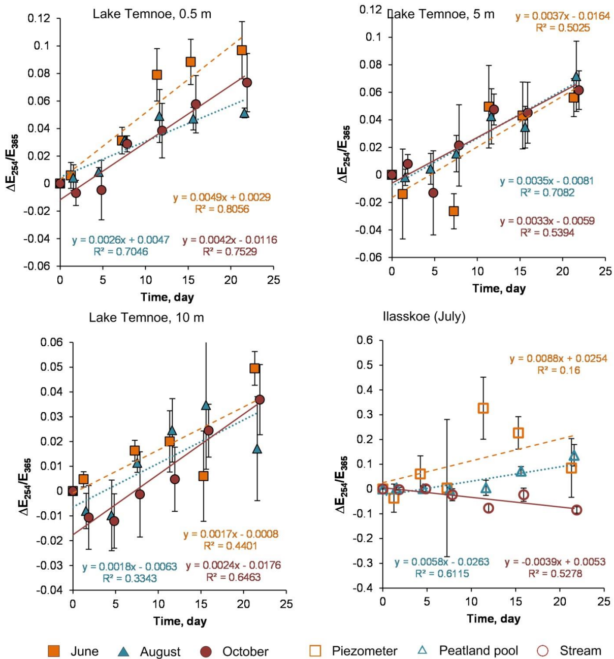
Fig. S3. The change of optical ratios ( E_{254}/E_{365} ) over time in bio-degradation experiments. Lake Temnoe 0.5 m (A), 5 m (B) and 10 m (C) in June (squares), August (triangles) and October (circles). Ilasskoe continuum in July (D) includes piezometer (squares), peatland pool Severnoe (triangles) and stream Chernyi (circles)
