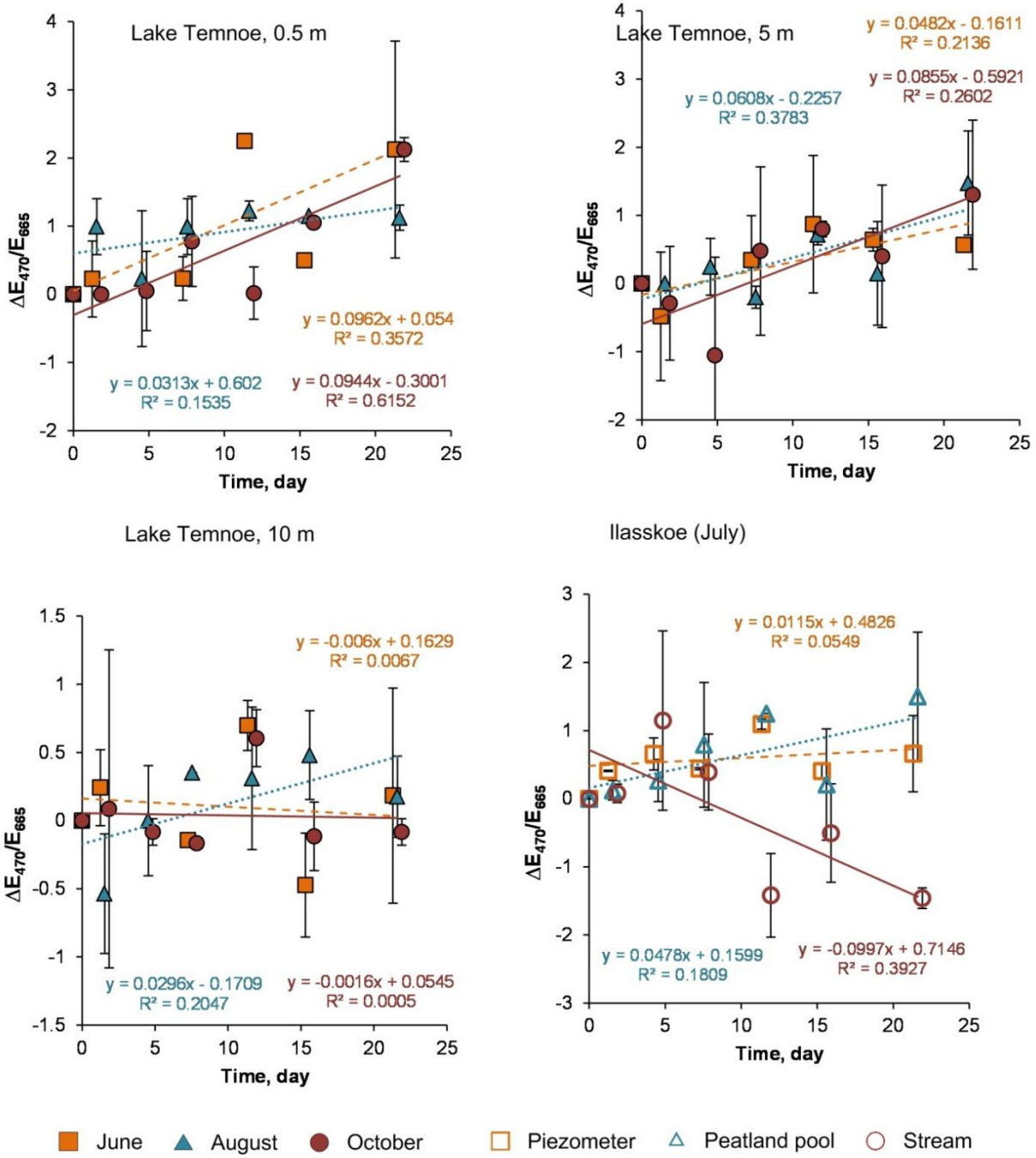
Fig. S3 , continued. The change of optical ratios ( E_{470}/E_{665} ) over time in bio-degradation experiments. Lake Temnoe 0.5 m (A), 5 m (B) and 10 m (C) in June (squares), August (triangles) and October (circles). Illasskoe continuum in July (D) includes piezometer (squares), peatland pool Severnoe (triangles) and outlet stream Chernyi (circles)
