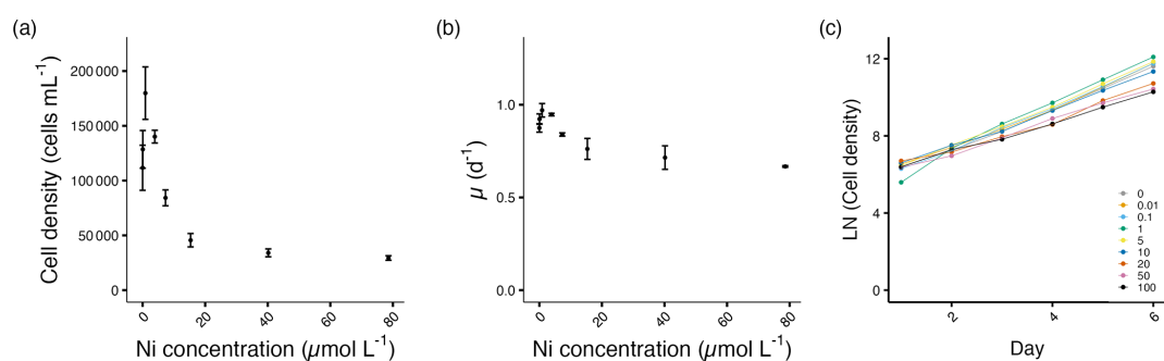
Figure 3. Growth performance of E. huxleyi . (a) Cell densities (cells mL -1 ) and (b) growth rates (d -1 ) plotted against measured Ni concentrations on the final experimental day. (c) Log-transformed cell densities plotted against time (day) to indicate the time of response; target Ni concentrations (μmol L -1 ) were used for clarity. Error bars denote standard deviations ( N = 3 ). Note that the data point at 0.01 μmol L -1 was excluded in (a) and (b) due to a technical measurement error. If not visible, error bars are smaller than the symbols.
