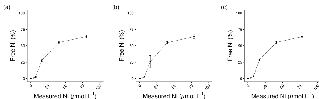
Figure 1. Percentage of free Ni 2+ in (a) A. carterae , (b) E. huxleyi , and (c) T. weissflogii cultures at the end of the experiment. Error bars denote standard deviations ( N = 3 ).
