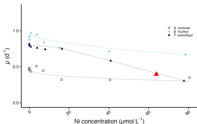
Figure 5. Predicted growth curves plotted against measured Ni concentrations. The red triangle denotes the IC50 value of T. weissflogii . Note that the predicted IC50 values of A. carterae and E. huxleyi are not shown as they exceed the highest tested Ni concentration.
