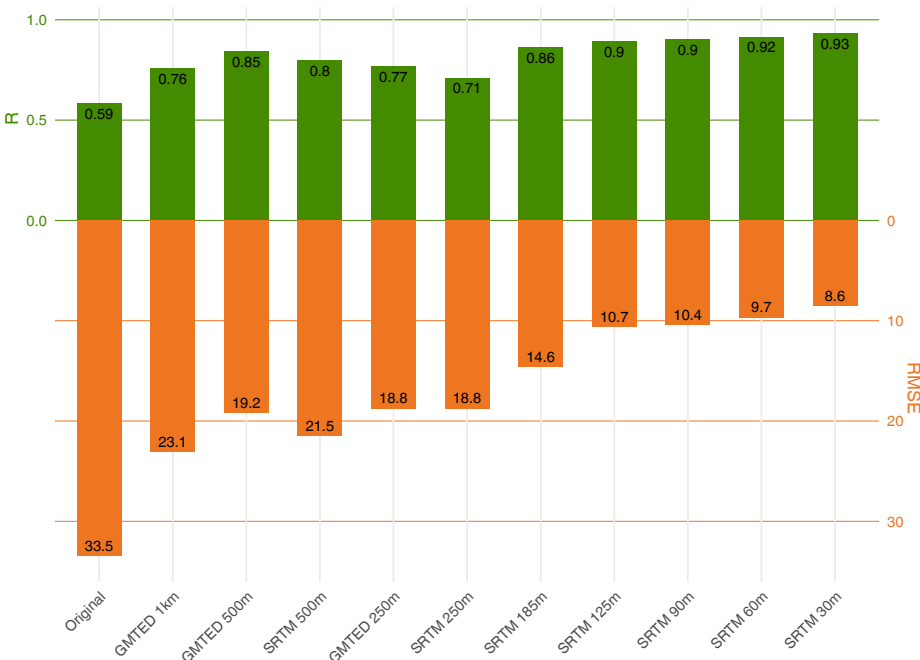
Barplot of R and RMSE for each DEM resolution
