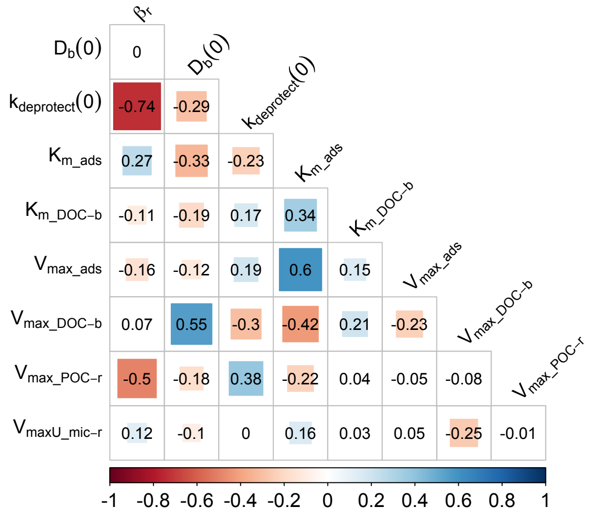
(b) Calibrated based on C and \delta^{13}C and \Delta^{14}C
