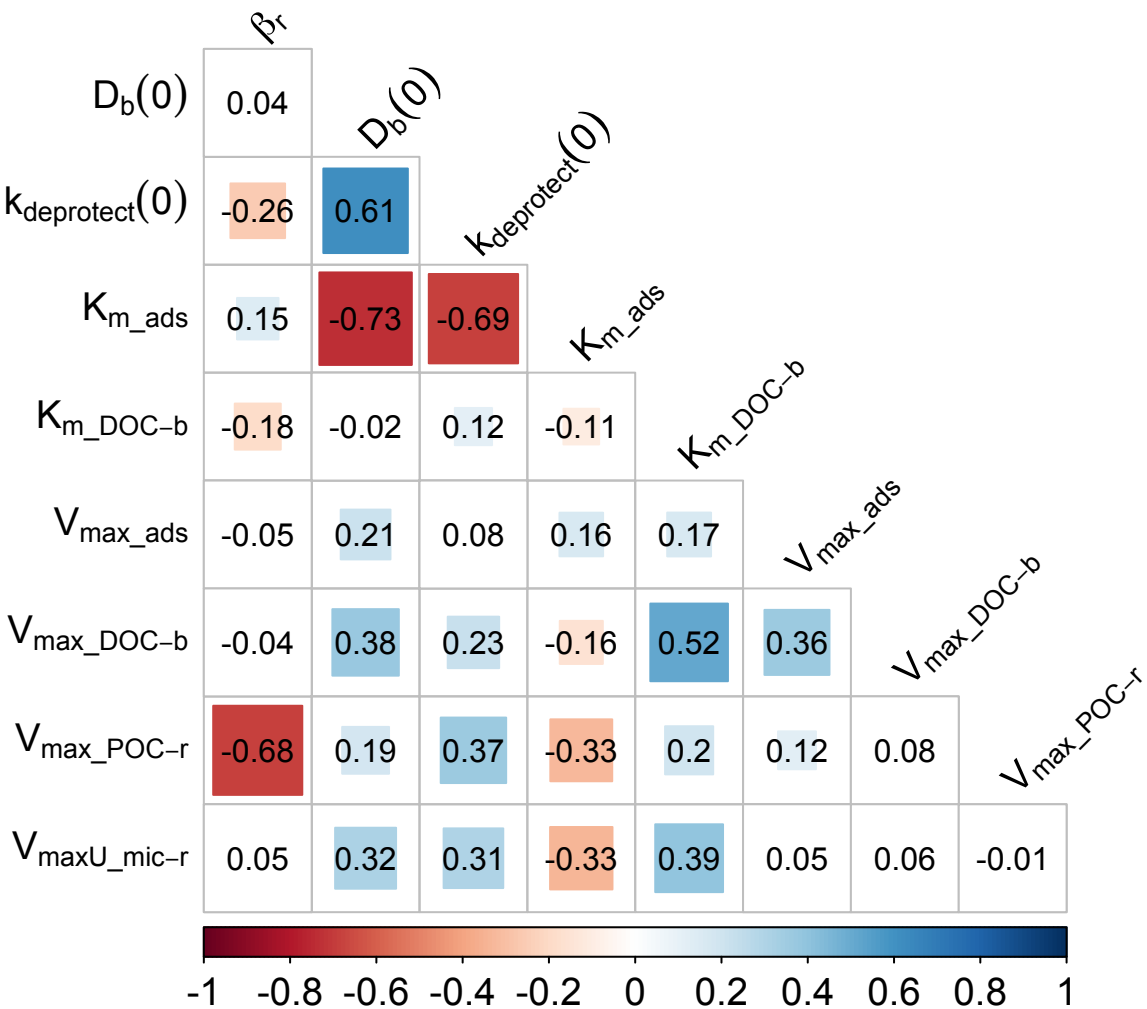
(a) Calibrated based on C
