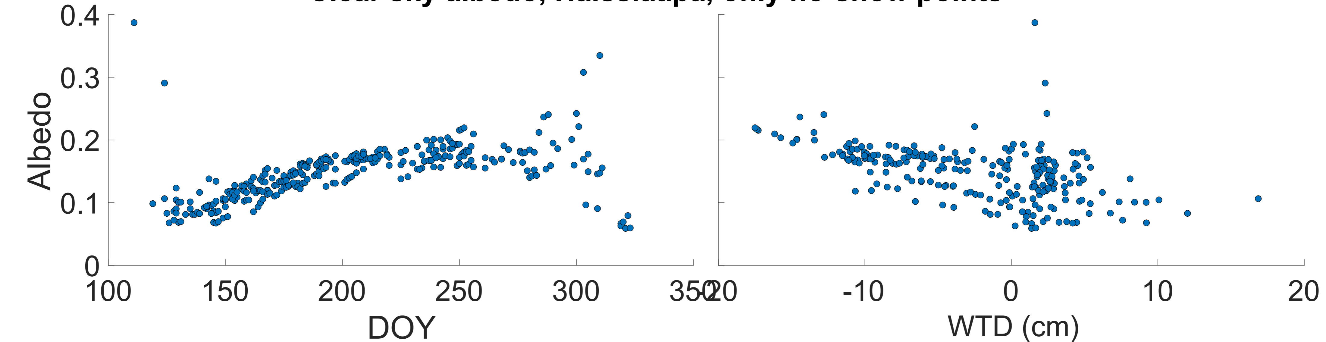
Clear sky albedo, Halssiaapa, only no-snow points
