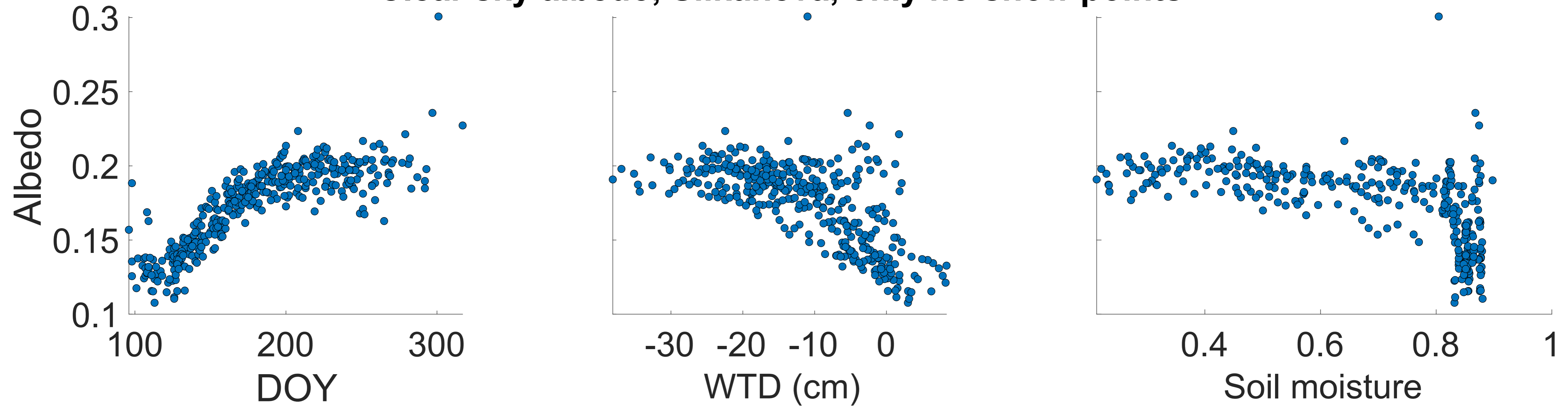
Clear sky albedo, Siikaneva, only no-snow points
