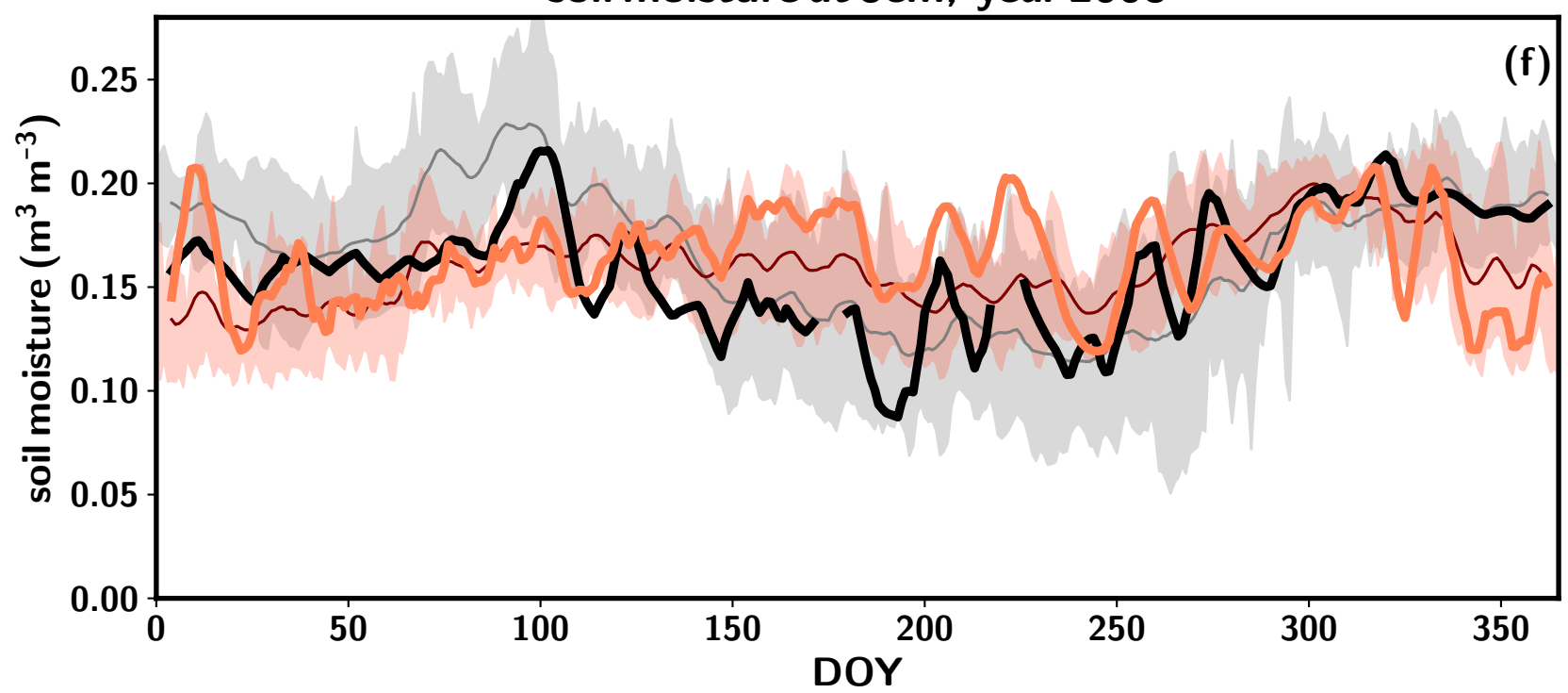
soil moisture at 5cm, year 2008
