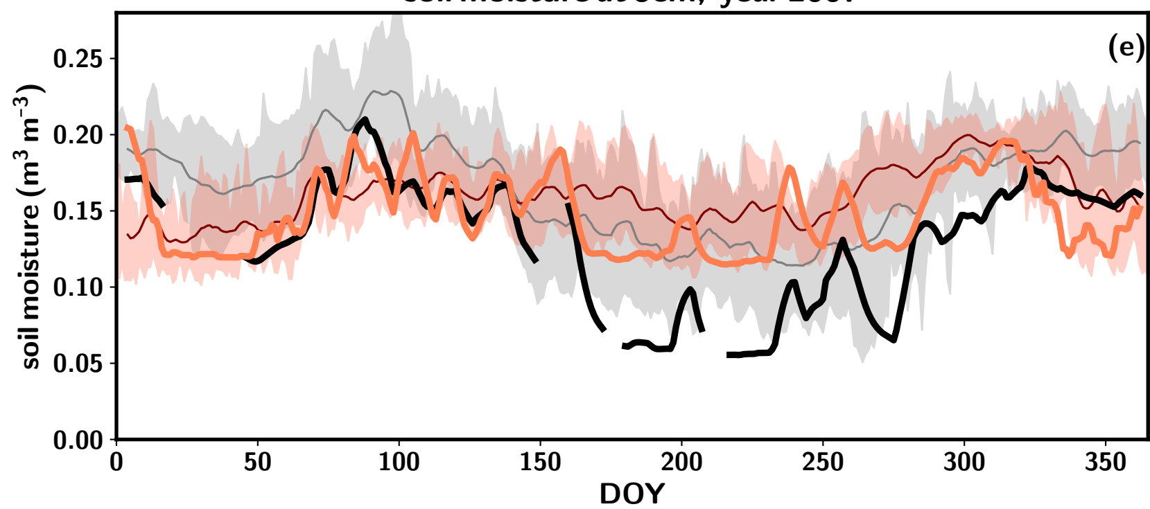
soil moisture at 5cm, year 2007
