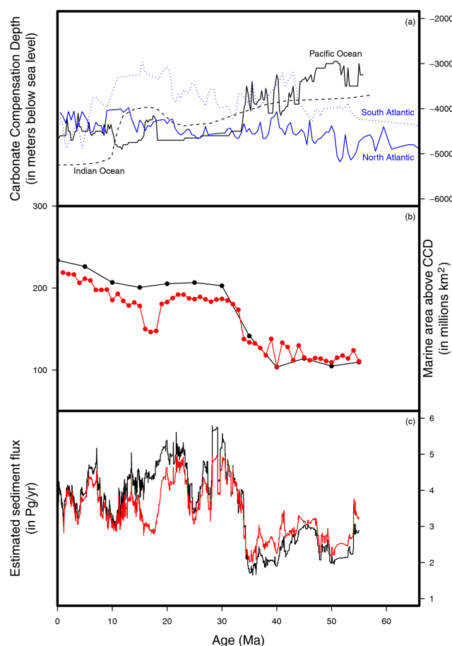
Figure 9. (a) CCD history for each basin, in metres below sea level (Van Andel, 1975; Pälike et al., 2012; Dutkiewicz and Müller, 2022). (b) Estimate of changes in the global depositional area of pelagic sediments, i.e. area above the carbonate compensation depth (CCD), expressed in millions of square kilometres ( \text{km}^2 ). Calculated from the CCD above and the paleobathymetric maps of Scotese and Wright (Scotese and Wright, 2018; Kocsis and Raja, 2020) in black and of Straume et al. (2024) in red. (c) Estimated flux of sediments throughout the Cenozoic, expressed in \text{Pg yr}^{-1} , based on the median SAR of each basin (Fig. 8) and the changes in depositional area of each basin.
