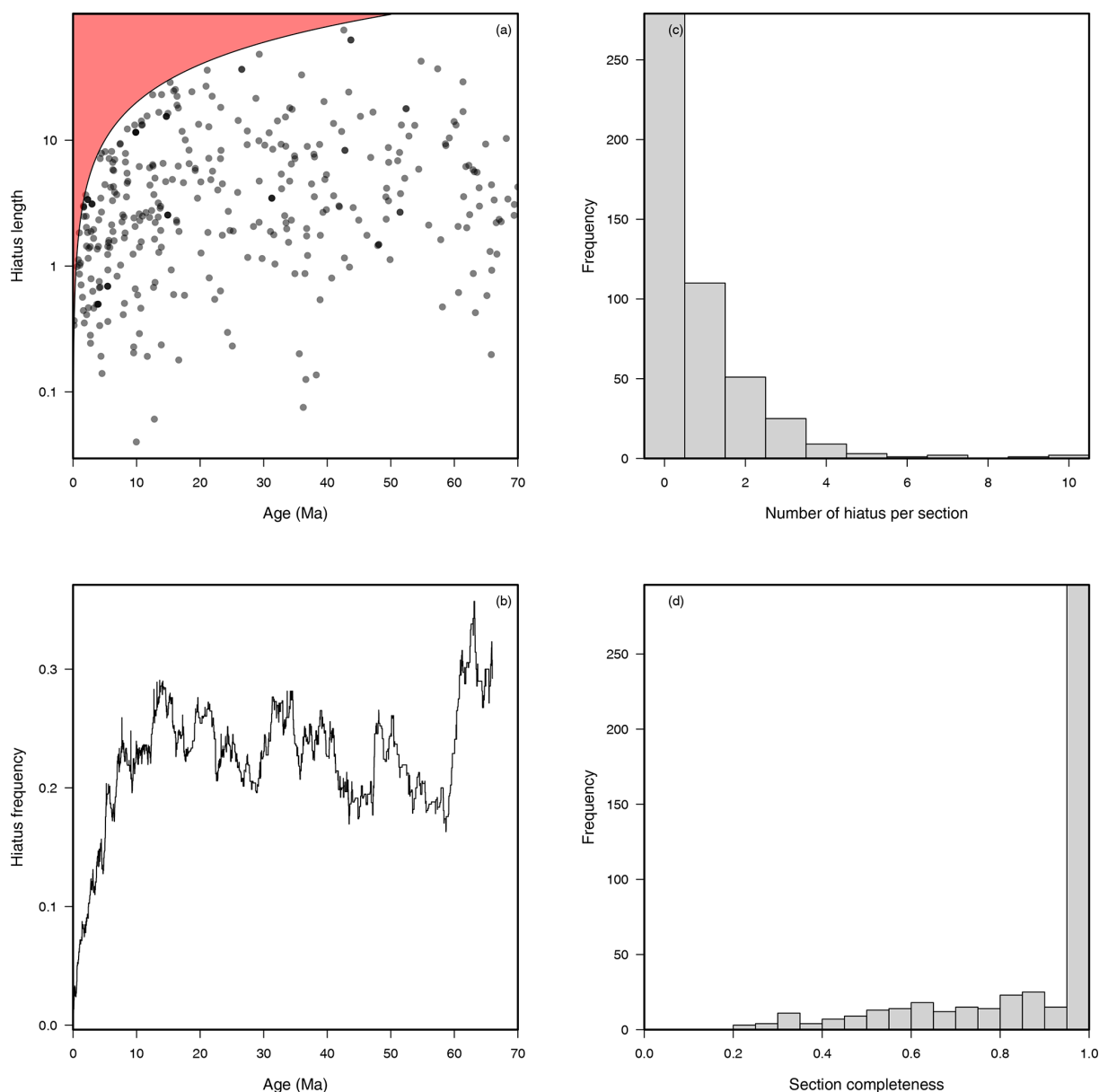
Figure 3. (a) Hiatus length through time (the age of the hiatus is its median age; in red is the area of the plot that thus can not be populated). (b) Hiatus frequency through time (i.e. what proportion of sections ranging through a given time interval do not recover that particular time interval). (c) Histogram of the number of hiatuses per section. (d) Histogram of section completeness (i.e. given a hole whose bottom core is at age x and what percentage of the x Ma was recovered).
