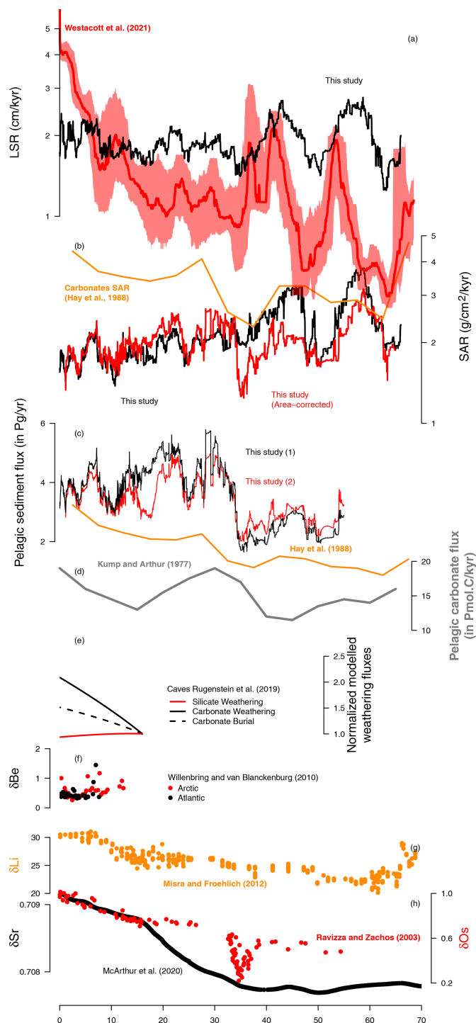
Figure 10. Comparison between various proxies and model outputs for Cenozoic weathering and reconstructed sediment accumulation rates or fluxes from the literature and this study. (a) LSR reconstructed here (in black) and in Westacott et al. (2021) (in red, with confidence interval). (b) SAR reconstructed in this study (in black from Fig. 7 and in red, area-corrected, from Fig. 8) and carbonates' SAR from Hay et al. (1988) (in orange). (c) Pelagic sediment flux reconstructed here (from Fig. 9, in black using Scotese and Wright paleobathymetry and in red using Straume et al. paleobathymetry) and in Hay et al. (1988) (in orange). (d) Pelagic carbonate flux reconstructed in Kump and Arthur (1977). (e) Modelled carbonate (in black) and silicate (in red) weathering fluxes and carbonate (dashed line) burial flux from Caves Rugenstein et al. (2019). (f–h) Weathering proxies: beryllium isotopes (f) from Willenbring and van Blanckenburg (2010), lithium isotopes (g) from Misra and Froehlich (2012), osmium isotopes (h, in red) from Ravizza and Zachos (2003), and strontium isotopes (h, in black) from McArthur et al. (2020).
