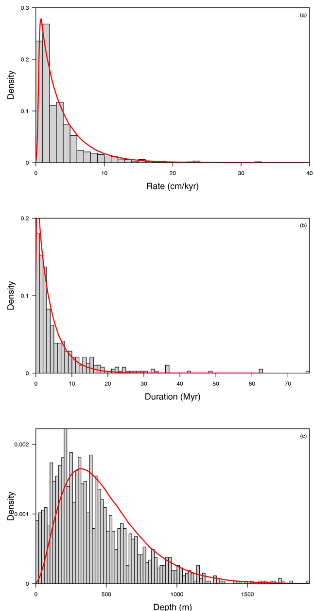
Figure 6. (a) Histogram of observed values of Pleistocene LSR in grey and density distribution of the modelled LSR (a translated Weibull distribution of shape \kappa = 0.95 , scale \lambda = 3.34 , and location \theta = 0.4 ) in red. (b) Histogram of observed hiatuses' duration in grey and density of the modelled distribution (a Weibull distribution of shape \kappa = 0.95 and scale \lambda = 4 ). (c) Histogram of DSDP, ODP, and IODP hole depths in grey and density of the modelled distribution (a Gamma distribution of shape \kappa = 2.93 and scale \theta = 166.97 ).
