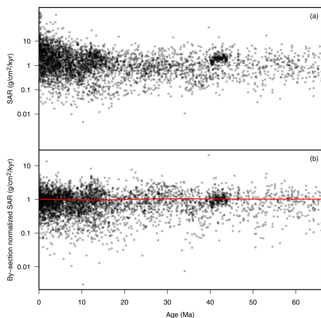
Figure 5. (a) SAR through time for each individual age model segment of a hole, compiled across all study holes' age models. (b) Same but for the SAR of each segment normalized by the mean SAR of its hole. Trend over time (LOESS; in red), showing the absence of a global pattern, on a hole by hole basis, toward increasing SAR over the Cenozoic.
