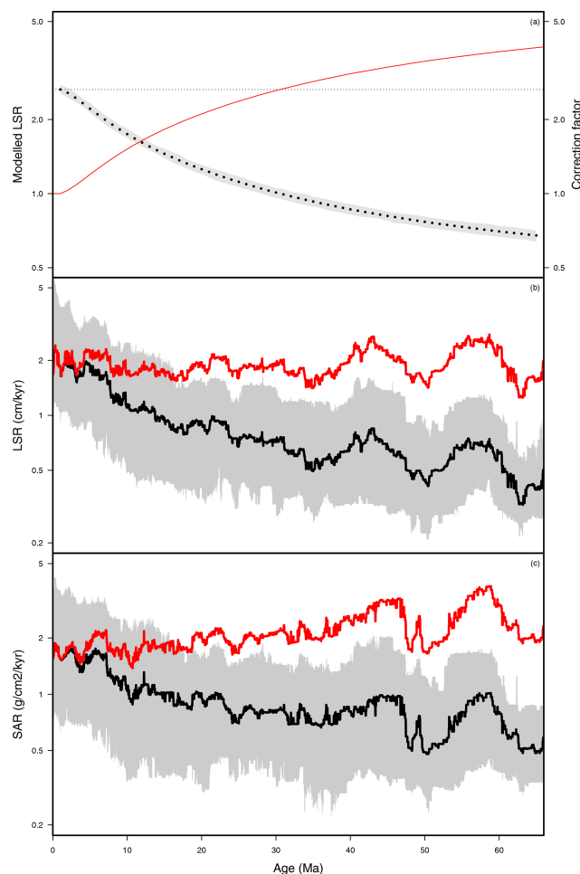
Figure 7. (a) Bias towards lower apparent sedimentation rate in older time intervals in drilled sections. Results from a model where there is no actual change in local accumulation rate over time and rates vary geographically. These sediments are then sampled by drilling sites with a randomly chosen drilling depth, drawn from the distribution of drilling depths of all deep-sea drilling programme sites. The apparent sedimentation rate over time compiled from the drilled sections is not constant but declines with increasing geological age, in part due to sediment compaction, but primarily by biased sampling of the older record. In black is the median LSR averaged over 1000 runs (in grey is the full extent of the various runs), the dotted line is the actual median LSR inputted in the model, and in red is the correction factor derived from it. (b, c) Linear sedimentation rates (b; expressed in \text{cm kyr}^{-1} ) and sediment accumulation rates (c; expressed in \text{g cm}^{-2} \text{kyr}^{-1} ). Black: distribution as observed in our global dataset (solid line: median; grey shading: interquartile range). Red: median sedimentation and accumulation rates corrected for drilling bias using the result of the model. Rates are given on a log scale.
