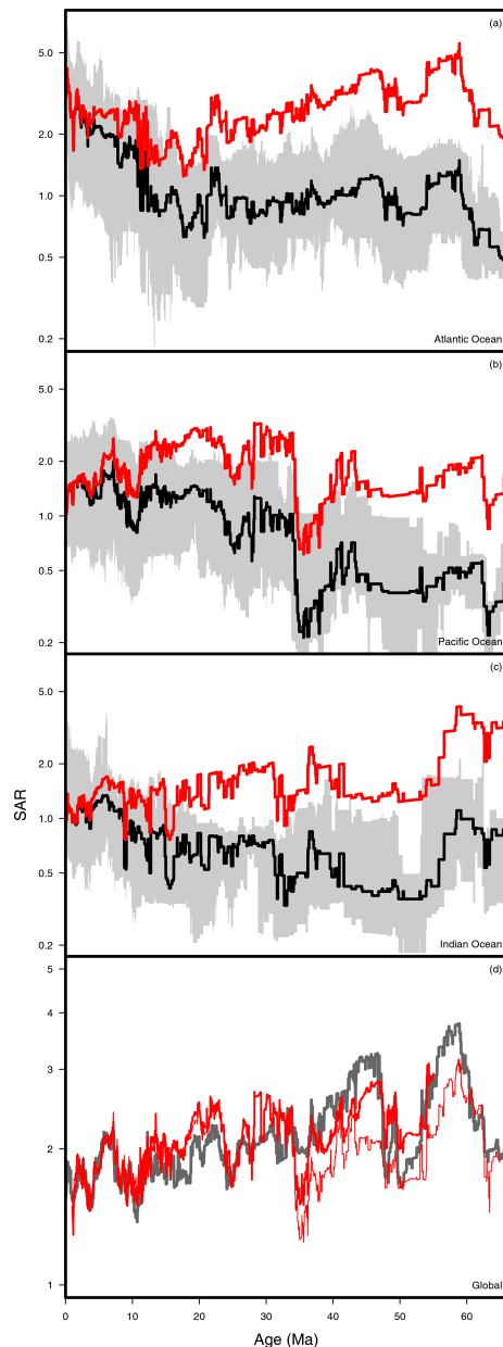
Figure 8. Sediment accumulation rate (expressed in \text{g cm}^{-2} \text{kyr}^{-1} ) distribution observed in each ocean basin (panels a–c; black: median; grey: interquartile range; red: median corrected for drilling bias using the result of the model), shown here on a log scale. Panel (d) shows the weighted global composite based on each basin's corrected median value (in bold red: full marine area; in dotted red: red-clay-free) compared to the corrected, but not area-weighted, global median SAR shown in Fig. 7.
