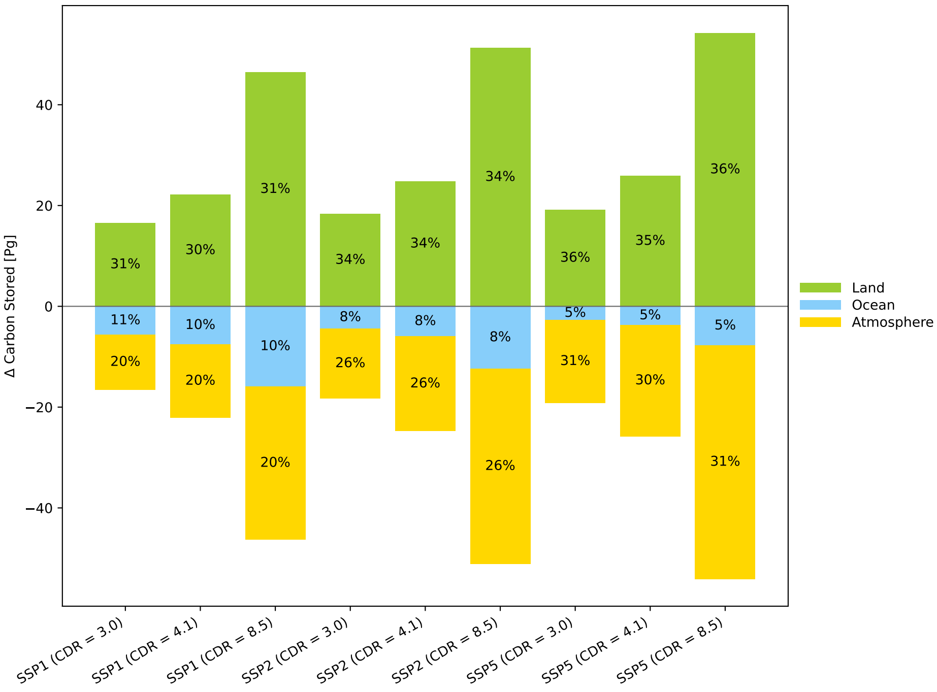
EOC Difference in Carbon Stored Between CDR and no-CDR Scenarios
