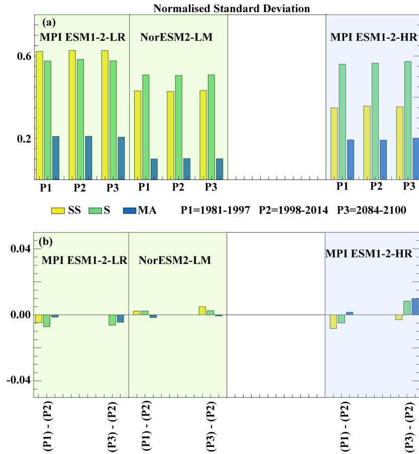
Figure S2: (a) Normalised standard deviation of SCHl from three different periods of piControl simulations (1981-1997, 1998-2014 & 2084-2100). (b) Difference between different periods considered. Shading in panel a and b represents the different model groups described in Section 3.2, with green for Group 1, and blue for Group 3.
