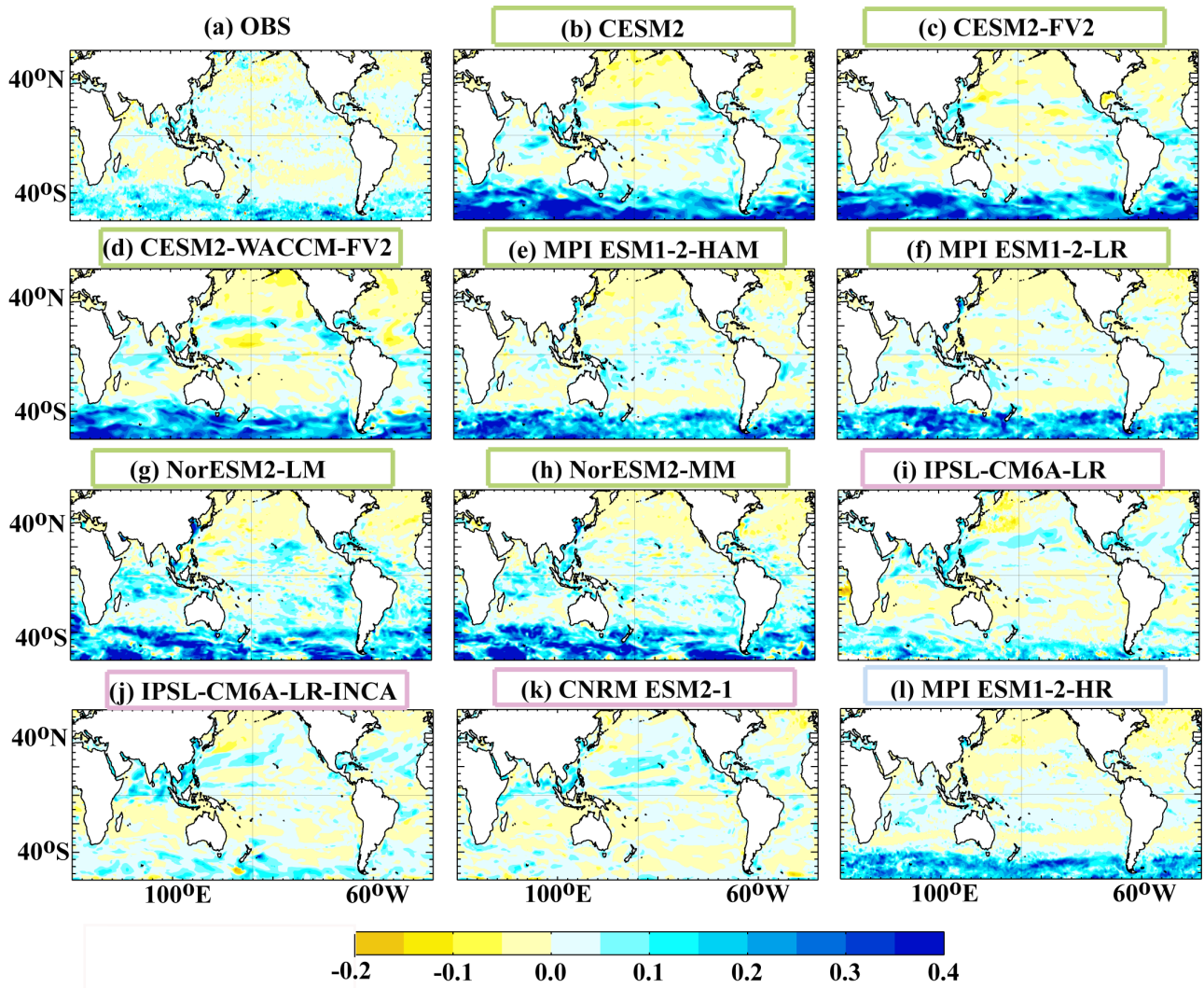
Figure S1: Regression of annual mean SCHl values on annual mean sub-seasonal values. Coloured boxes for the model names represent the different model groups described in Section 3.2, with green for Group 1, pink for Group 2, and blue for Group 3.
