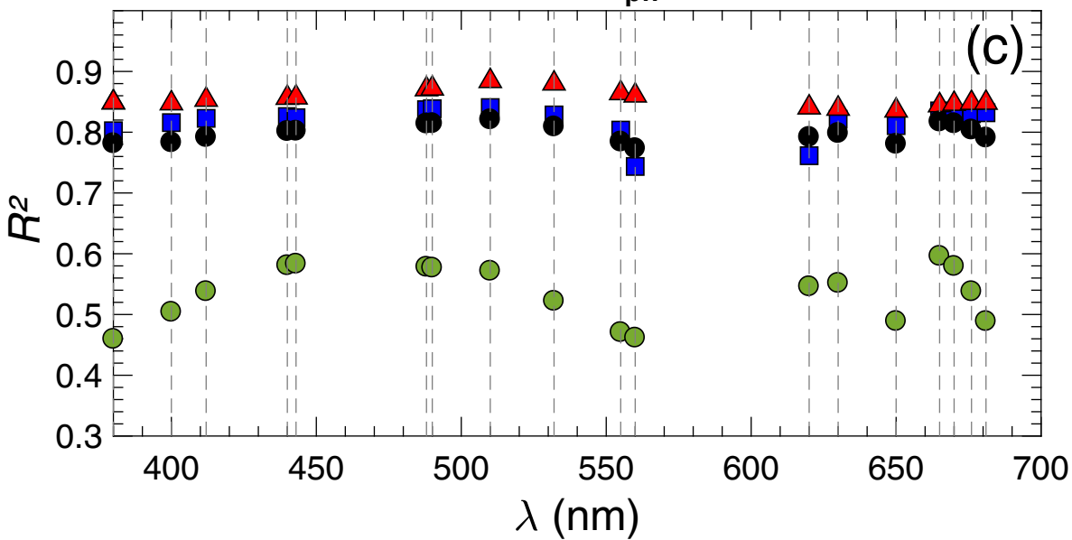
PON vs. a_{ph}(\lambda)
