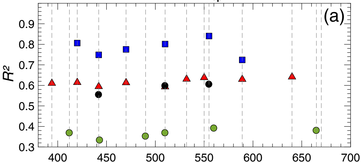
PON vs. b_{bp}(\lambda)
