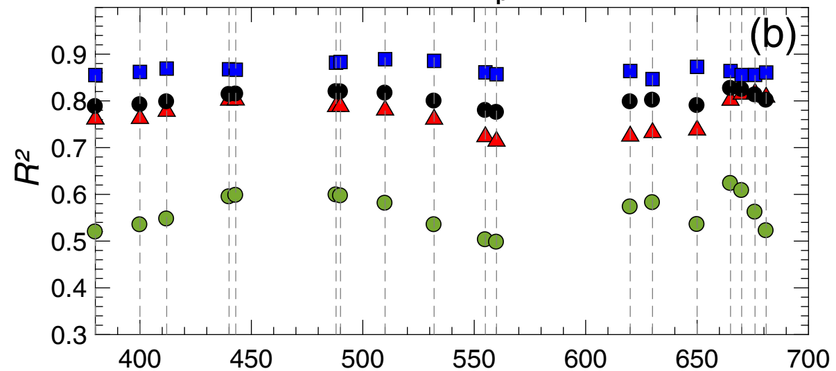
PON vs. a_p(\lambda)
