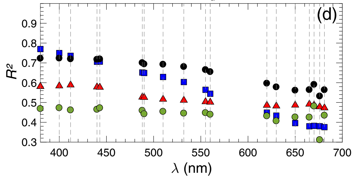
PON vs. a_d(\lambda)
