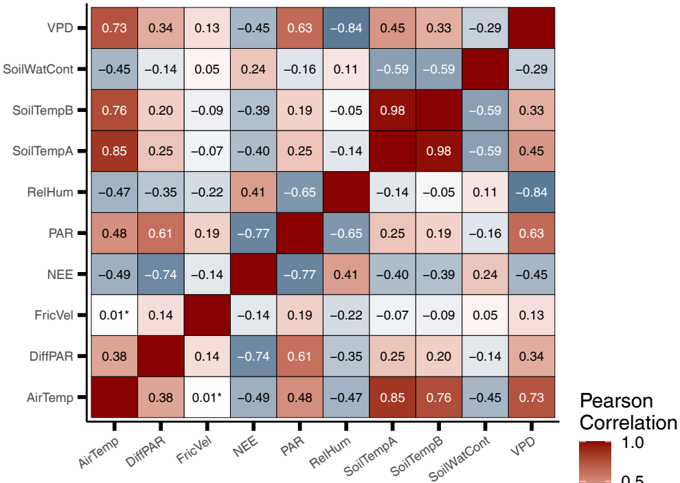
Correlation Matrix for Hyytiälä
