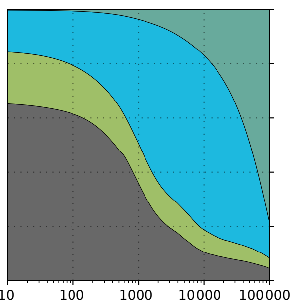
(c) 5000 PgC
