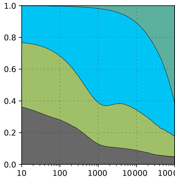
(a) 500 PgC
