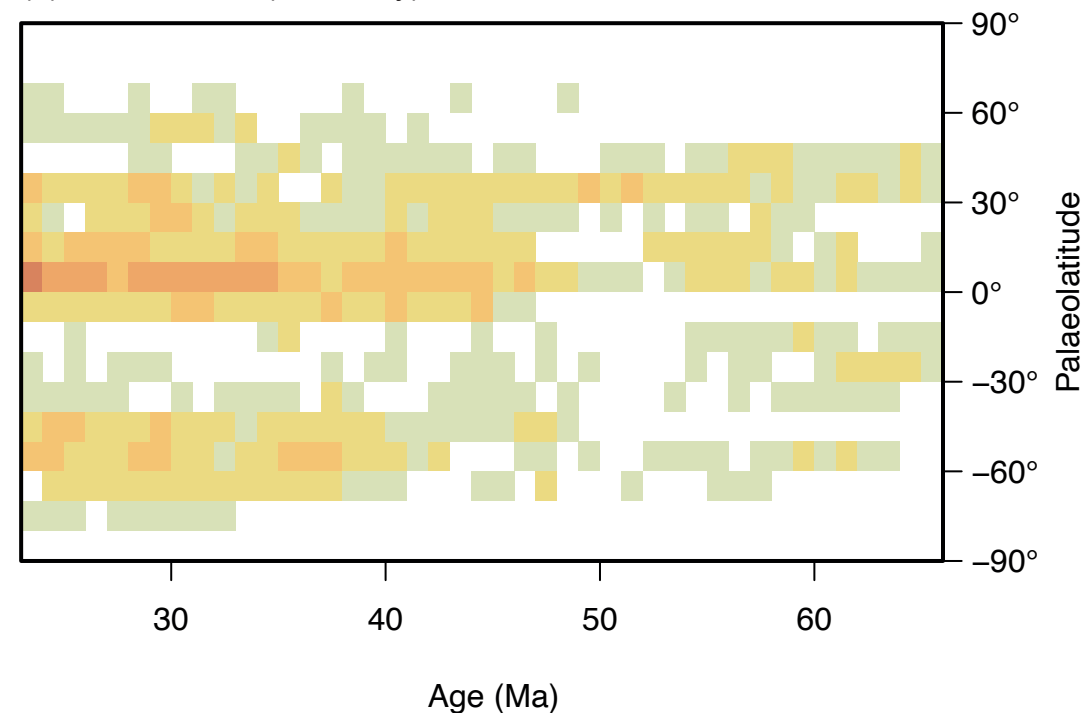
(b) Radiolarians (this study)
