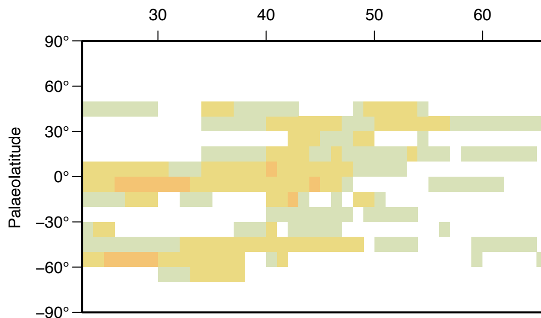
(c) Cherts (this study)
