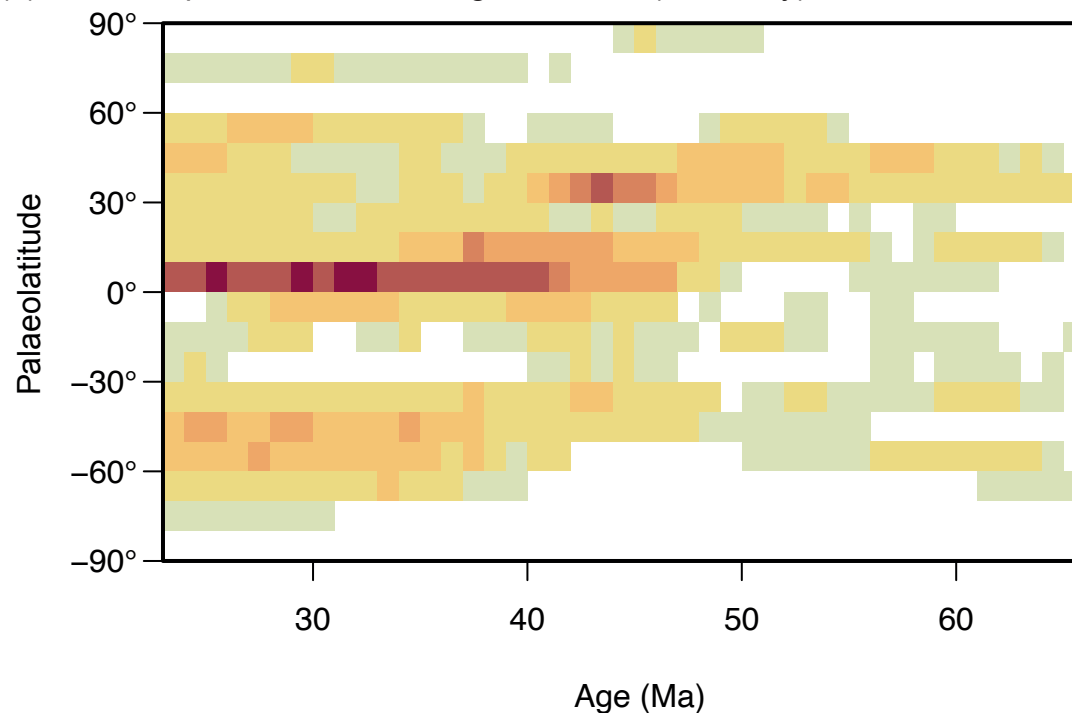
(a) Total deep-sea diatom-bearing sediments (this study)
