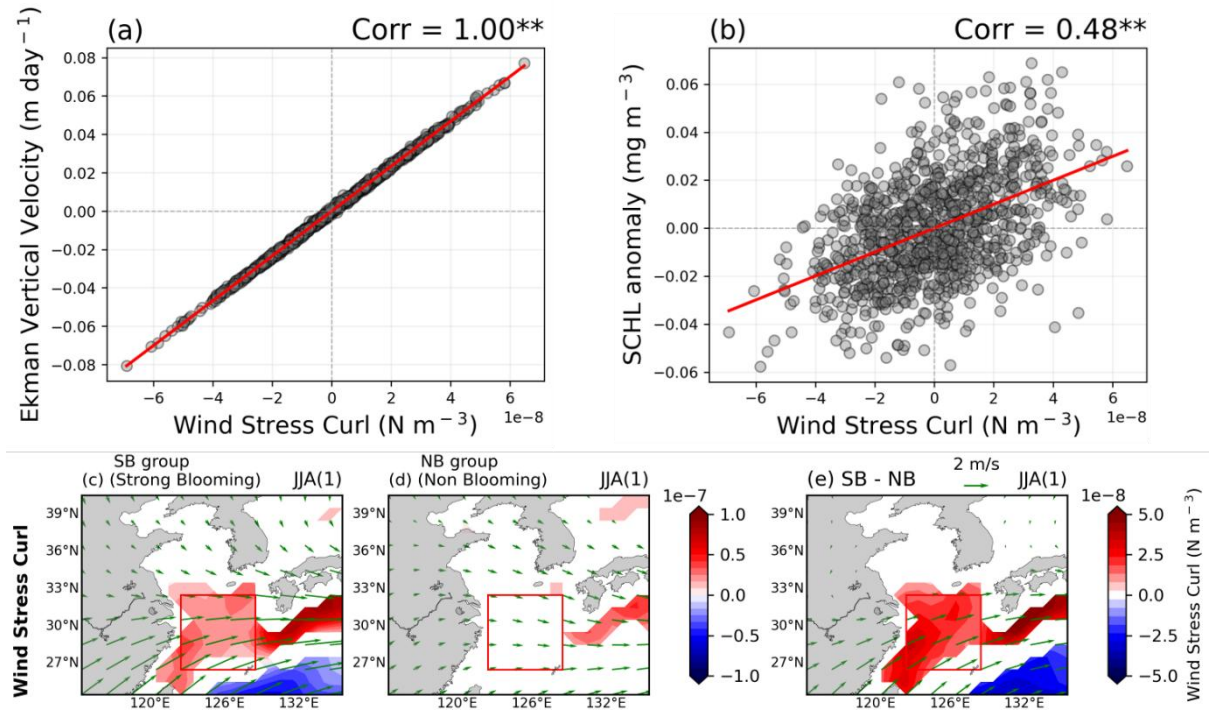
Figure S2. (a) The relationship between area-averaged Wind Stress Curl (WSCL) and Ekman Upwelling (EKU) in the target area during the post-El Niño summers. (b) The relationship between area-averaged Wind Stress Curl (WSCL) and SCHL anomalies in the target area during the post-El Niño summers. (c-e) Composite maps exhibiting the EKU anomalies during the post-El Niño summer season for both groups, as well as the difference between the two groups. All the shadings and vectors are expressed only in the region where the responses are statistically significant at the 95% confidence level.
