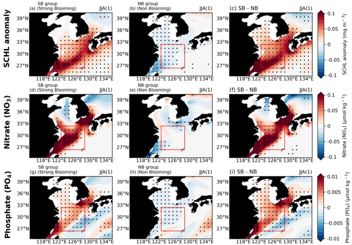
Figure S1. (a-c) Composite maps exhibiting the 3-month average of Surface Chlorophyll-a (SCHL) anomalies for the Strong Blooming (SB) group, Non-Blooming (NB) group and the difference between the two groups during the post-El Niño summers. (d-f) Composite maps exhibiting the surface nitrate ( \text{NO}_3 ) anomalies of the SB group, NB group and difference between the two groups during the post-El Niño summers. (g-i) Composite maps exhibiting the surface phosphate ( \text{PO}_4 ) anomalies of the SB group, NB group and the difference between the two groups during the post-El Niño summers. Black dots indicate the responses are statistically significant at the 95% confidence level by using the bootstrap method.
