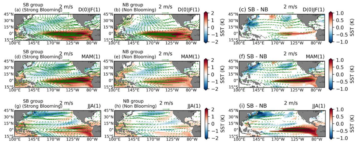
Figure S3. The figures exhibit the evolution map of Sea Surface Temperature (SST) anomaly patterns from the El Niño mature phase to the post-El Niño summer season. (a-c) Composite maps exhibiting the SST anomaly patterns for the SB, and NB group and the difference between the two groups during the El Niño mature phase. (d-f) Composite maps exhibiting the SST anomaly patterns for the SB, and NB group and the difference between the two groups during the following spring season of the El Niño mature phase. (g-i) Composite maps exhibiting the SST anomaly patterns of the SB, and NB group and the difference between the two groups during the post-El Niño summers. All the shadings and vectors are expressed only in the region where the responses are statistically significant at the 95% confidence level.
