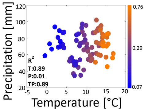
LPJ-Guess
