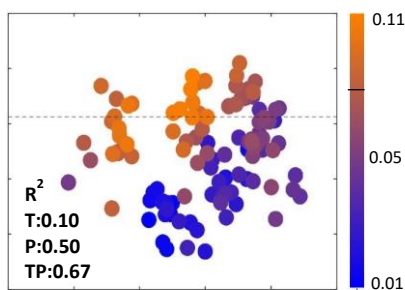
LPX-Bern
