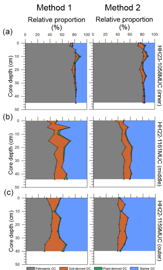
Figure 9. Depth profiles showing the relative proportions of petrogenic, soil-derived, plant-derived, and marine OC, as determined using Method 1 (based on \delta^{13}\text{C}_{\text{org}} (‰ VPDB), \Delta^{14}\text{C}_{\text{org}} (‰), and (\text{Ad}/\text{Al})_v ratio) and Method 2 (based on \delta^{13}\text{C}_{\text{org}} (‰ VPDB), \Delta^{14}\text{C}_{\text{org}} (‰), and lignin phenols ( \text{mg gOC}^{-1} )), for the cores (a) HH23-1058MUC, (b) HH22-1161MUC, and (c) HH22-1159MUC.
