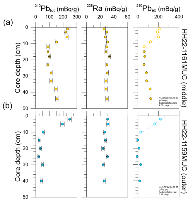
Figure 3. Depth profiles of ^{210}\text{Pb}_{\text{tot}} ( \text{mBq g}^{-1} ), ^{226}\text{Ra} ( \text{mBq g}^{-1} ), and ^{210}\text{Pb}_{\text{ex}} ( \text{mBq g}^{-1} ) for the cores (a) HH22-1161MUC and (b) HH22-1159MUC. Open circles indicate the data points used in the linear regressions (yellow and blue dotted lines) of the natural log-transformed ^{210}\text{Pb}_{\text{ex}} versus depth, which were applied to estimate sedimentation rates.
