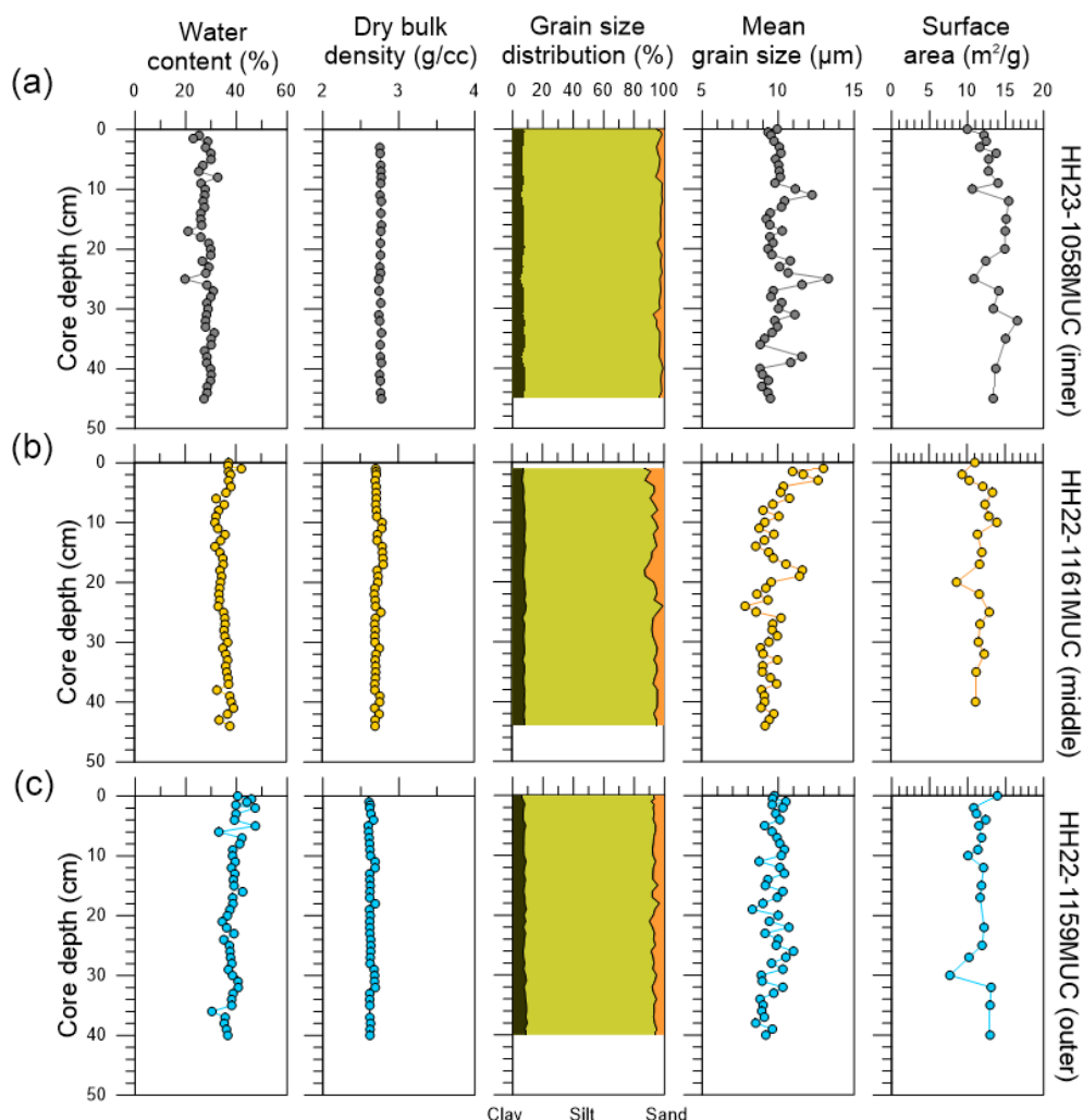
Figure 2. Depth profiles of water content (%), dry bulk density ( \text{g cm}^{-3} ), grain size distribution (%), mean grain size ( \mu\text{m} ), and surface area ( \text{m}^2 \text{g}^{-1} ) for the cores (a) HH23-1058MUC, (b) HH22-1161MUC, and (c) HH22-1159MUC.
