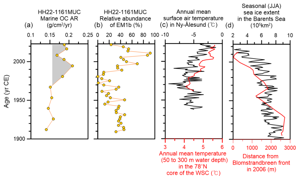
Figure 11. Age profiles of (a) the accumulation rates of marine OC based on Method 2 for core HH22-1161MUC, (b) the relative abundance (%) of EM1b for core HH22-1161MUC, (c) annual mean surface air temperatures (°C) in Ny-Ålesund (black; data from MOSJ, environmental monitoring of Svalbard and Jan Mayen) and integrated annual mean temperatures (°C) at 50–300 m water depth in the 78° N core of the West Spitsbergen Current (red; data from MOSJ), and (d) seasonal (JJA) sea ice extent in the Barents Sea (black; data from NSIDC; National Snow and Ice Data Center) and the distance from the Blomstrandbreen front in Kongsfjorden in 2006 (red; data from Burton et al., 2016).
