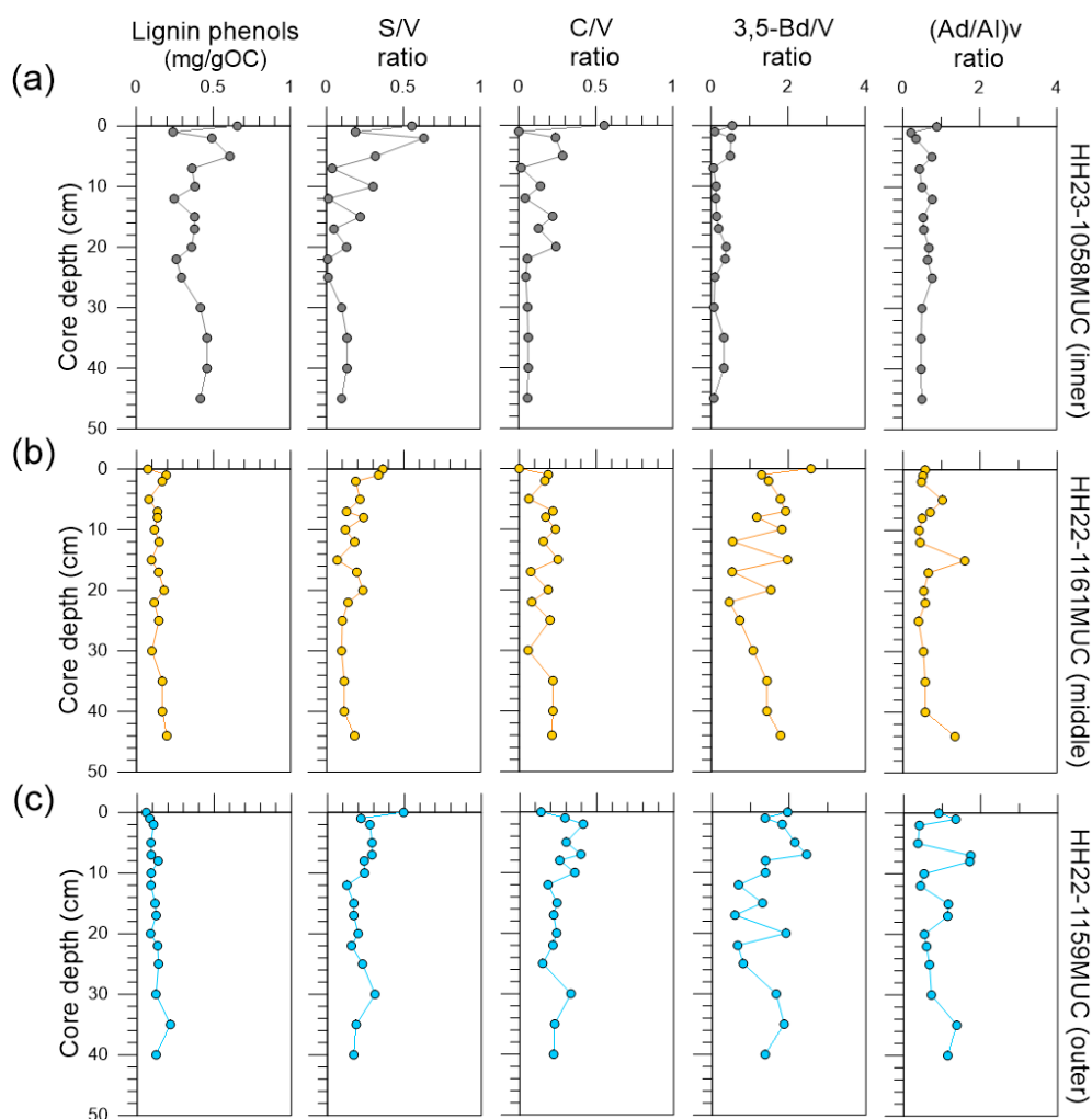
Figure 5. Depth profiles of lignin phenol concentrations ( \text{mg gOC}^{-1} ) and S / V, C / V, 3,5-Bd / V, and (\text{Ad} / \text{Al})_v ratios for the cores (a) HH23-1058MUC, (b) HH22-1161MUC, and (c) HH22-1159MUC.
