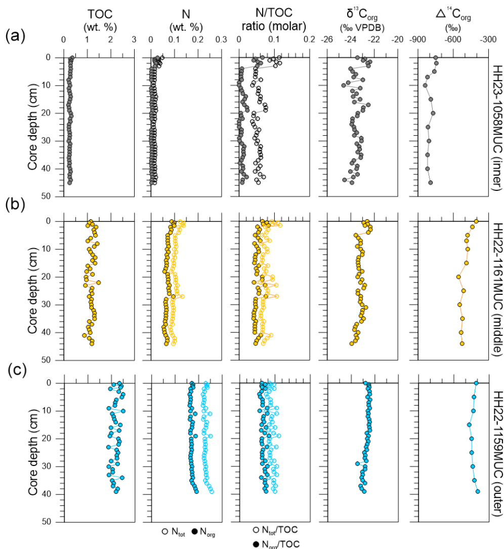
Figure 4. Depth profiles of TOC (wt %), N (wt %), N / TOC ratios (molar), \delta^{13}\text{C}_{\text{org}} (‰ VPDB), and \Delta^{14}\text{C}_{\text{org}} (‰) for the cores (a) HH23-1058MUC, (b) HH22-1161MUC, and (c) HH22-1159MUC.
