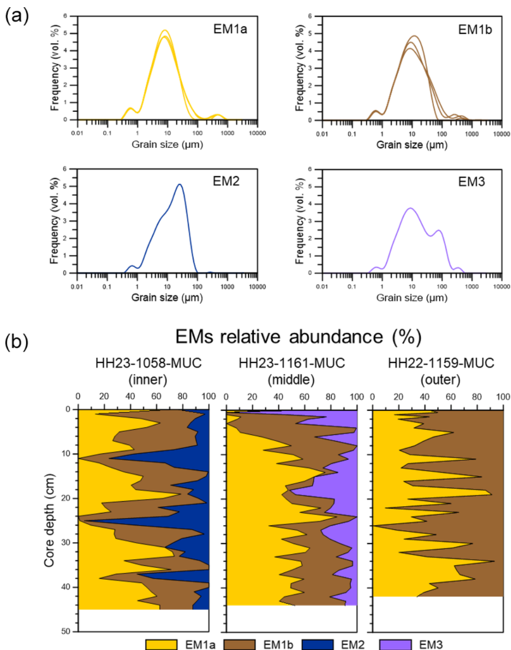
Figure 6. (a) Classified grain-size end-member distribution curves from three cores and (b) depth profiles showing the variation in the relative abundances of grain-size end-members (EM1a, EM1b, EM2, and EM3) in the three cores analyzed in this study.
