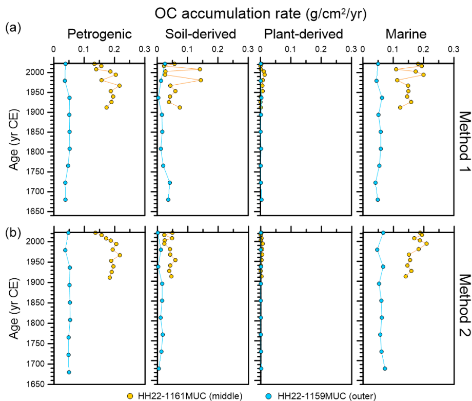
Figure 10. Age profiles of the accumulation rates (g cm -2 yr -1 ) of petrogenic, soil-derived, plant-derived, and marine OC, as determined using Method 1 (based on \delta^{13}\text{C}_{\text{org}} (‰ VPDB), \Delta^{14}\text{C}_{\text{org}} (‰), and (\text{Ad} / \text{Al})_v ratio) and Method 2 (based on \delta^{13}\text{C}_{\text{org}} (‰ VPDB), \Delta^{14}\text{C}_{\text{org}} (‰), and lignin phenols (mg / gOC)), for the cores HH23-1058MUC, HH22-1161MUC, and HH22-1159MUC.
