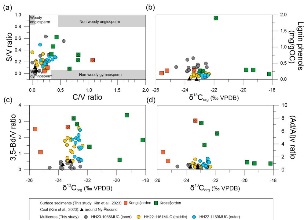
Figure 8. Scatter plots of (a) C / V ratio versus S / V ratio, including the end-members for different vascular plant tissues (cf. Goñi et al., 2000), (b) \delta^{13}\text{C}_{\text{org}} (‰ VPDB) versus lignin phenols ( \text{mg/g OC}^{-1} ), (c) \delta^{13}\text{C}_{\text{org}} (‰ VPDB) versus 3,5-Bd / V ratio, and (d) \delta^{13}\text{C}_{\text{org}} (‰ VPDB) versus (Ad / Al) v ratio for the three cores, compared with data from coals (Kim et al., 2023) and surface sediments (Kim et al., 2023, and this study). Note that the surface sediment samples newly analyzed in this study are indicated by hashed square symbols.
