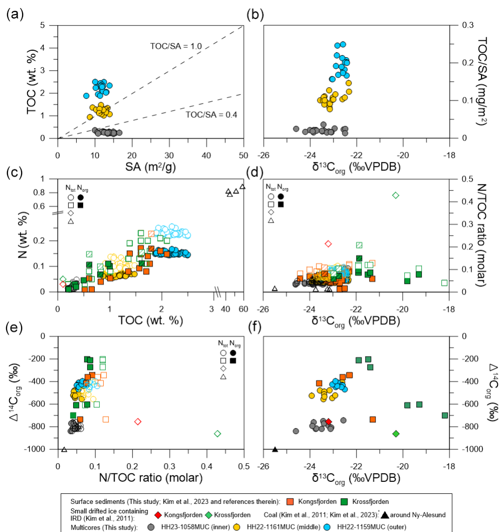
Figure 7. Scatter plots of (a) SA ( \text{m}^2 \text{g}^{-1} ) versus TOC (wt %), (b) \delta^{13}\text{C}_{\text{org}} (‰ VPDB) versus TOC / SA ( \text{mg m}^{-2} ), (c) TOC (wt %) versus N_{\text{tot}} or N_{\text{org}} (wt %), (d) \delta^{13}\text{C}_{\text{org}} (‰ VPDB) versus N_{\text{tot}} / TOC (molar) ratios or N_{\text{org}} / TOC (molar) ratios, (e) N_{\text{tot}} / TOC (molar) ratios or N_{\text{org}} / TOC (molar) ratios versus \Delta^{14}\text{C}_{\text{org}} (‰), and (f) \delta^{13}\text{C}_{\text{org}} (‰ VPDB) versus \Delta^{14}\text{C}_{\text{org}} (‰) for the three cores, compared with data from small drifted ice containing IRD (Kim et al., 2011), coals (Kim et al., 2011; Kim et al., 2023), and surface sediments (Kim et al., 2023, and this study). Note that the surface sediment samples newly analyzed in this study are denoted by hashed square symbols.
