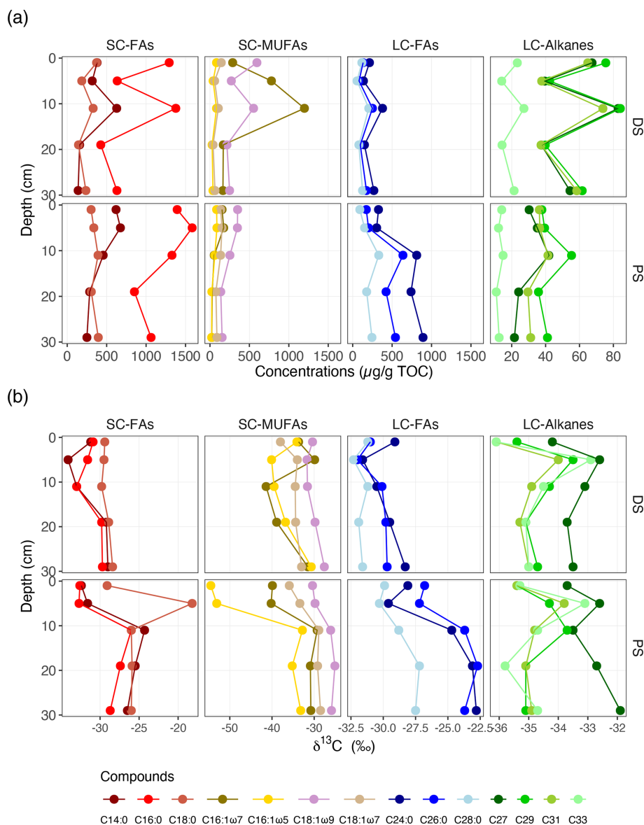
Figure 3. Vertical distribution of specific fatty acids and n -alkanes in deltaic (DS) and profundal (PS) sediments of Lake Geneva. (a) Concentrations (expressed as μg lipid g -1 TOC) and (b) compound-specific δ 13 C values (in ‰ vs. VPDB). SC-FAs denotes short-chain fatty acids (C 14:0 , C 16:0 , and C 18:0 ), SC-MUFAs denotes short-chain monounsaturated fatty acids (C 16:1 and C 18:1 ), LC-FAs denotes long-chain fatty acids (C 24:0 , C 26:0 , and C 28:0 ), and LC-alkanes denotes long-chain n -alkanes (C 27 , C 29 , C 31 , and C 33 ).
