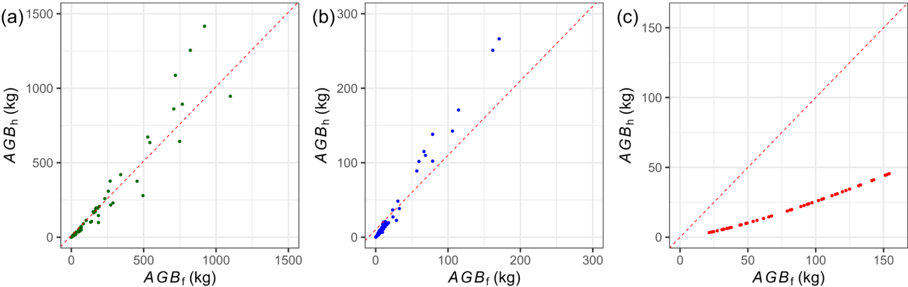
135 Figure S11. The 1:1 line plot comparison between aboveground biomass ( AGB , kg) estimated by the diameter at breast height ( DBH ) and height ( H ) relationship ( AGB_h , kg) and aboveground biomass estimated by adopted functions ( AGB_f , kg) for evergreen forests (EF) (a), regrowth forests (RF) (b), and cashew plantations (CP) (c).
