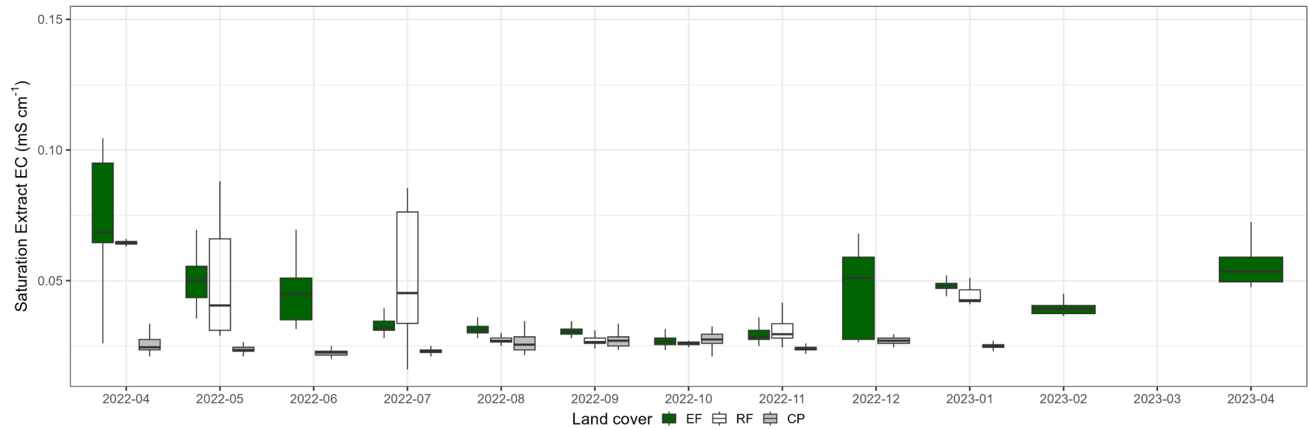
Figure S7. Monthly mean soil saturation extraction electrical conductivity ( \text{mS cm}^{-1} ) for different land-cover classes from April 10, 2022, to April 9, 2023. The mean values were calculated by averaging the data from two representative plots for each land-cover class. Soil sensors were installed 0.2 m below the ground.
