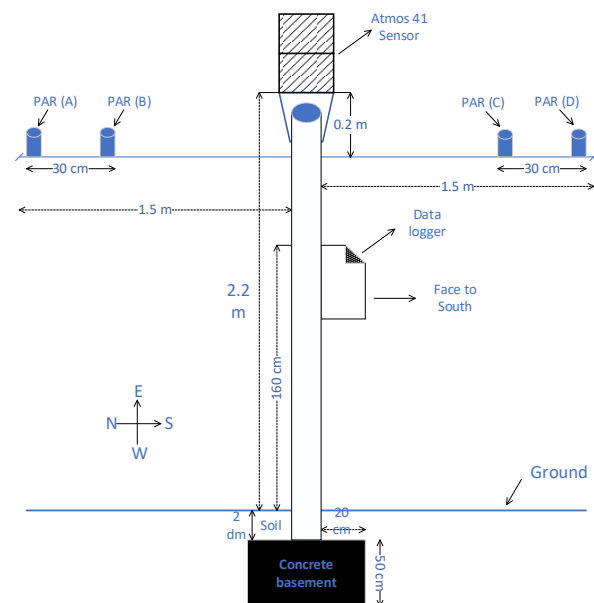
Figure S3. The diagram depicts the installation configuration of weather and photosynthetically active radiation ( PAR ) sensors at the Kulen Station. The weather sensor was installed at a height of 2.2 m above the ground, while the PAR sensors were placed at a height of 2 m above the ground.
