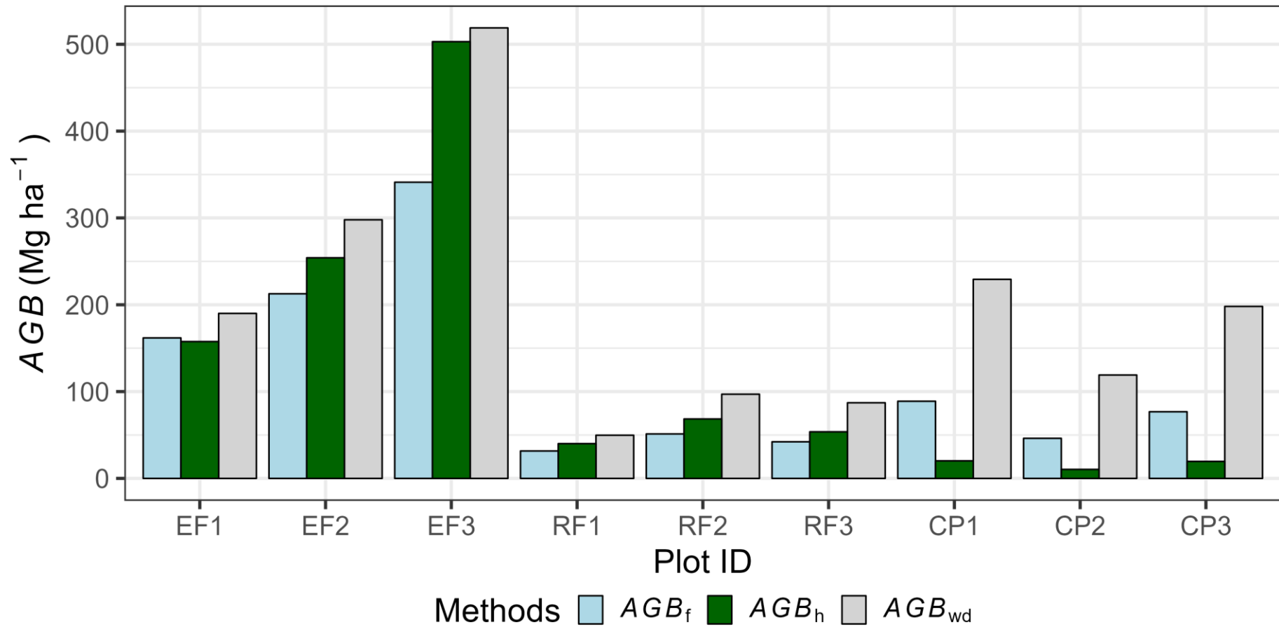
Figure S12. The estimation of aboveground biomass ( AGB ) (Mg ha -1 ) by different methods for each inventory plot. “ AGB_f ” represents aboveground biomass estimated by adopted functions; “ AGB_{wd} ” represents aboveground biomass estimated by adopted functions utilizing species-specific wood density; “ AGB_h ” represents aboveground biomass estimated by the diameter at breast height ( DBH ) and height ( H ) relationship, along with species-specific wood density, for our study site.
