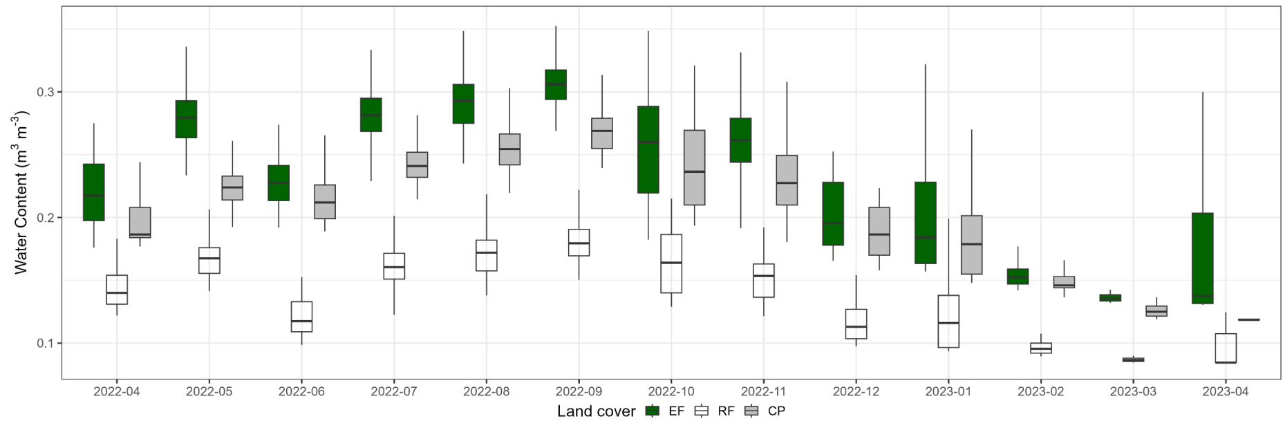
Figure S6. Monthly mean water content ( \text{m}^3 \text{m}^{-3} ) for different land-cover classes from April 10, 2022, to April 9, 2023. The mean values were calculated by averaging the data from two representative plots for each land-cover class. Soil sensors were installed 0.2 m below the ground.
