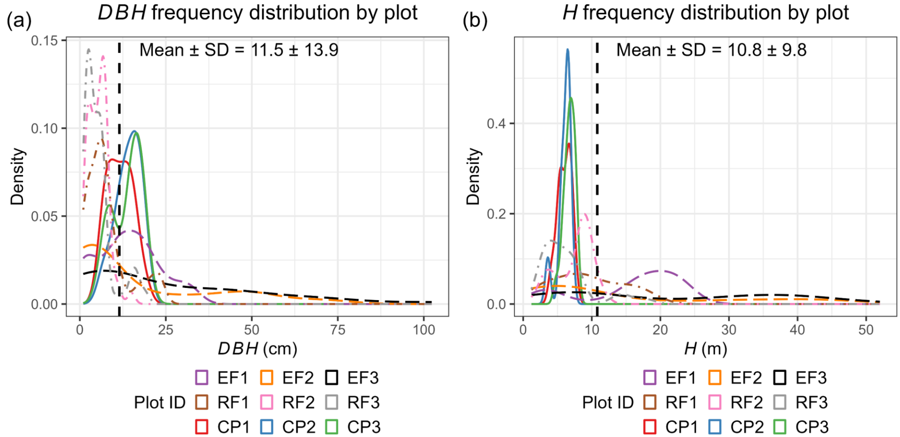
Figure S9. The frequency distributions of tree diameters at the breast height ( DBH , cm) and height ( H , m) across different plots. The plot labels “EF”, “RF”, and “CP” correspond to “evergreen forests”, “regrowth forests” and “cashew plantations” respectively.
