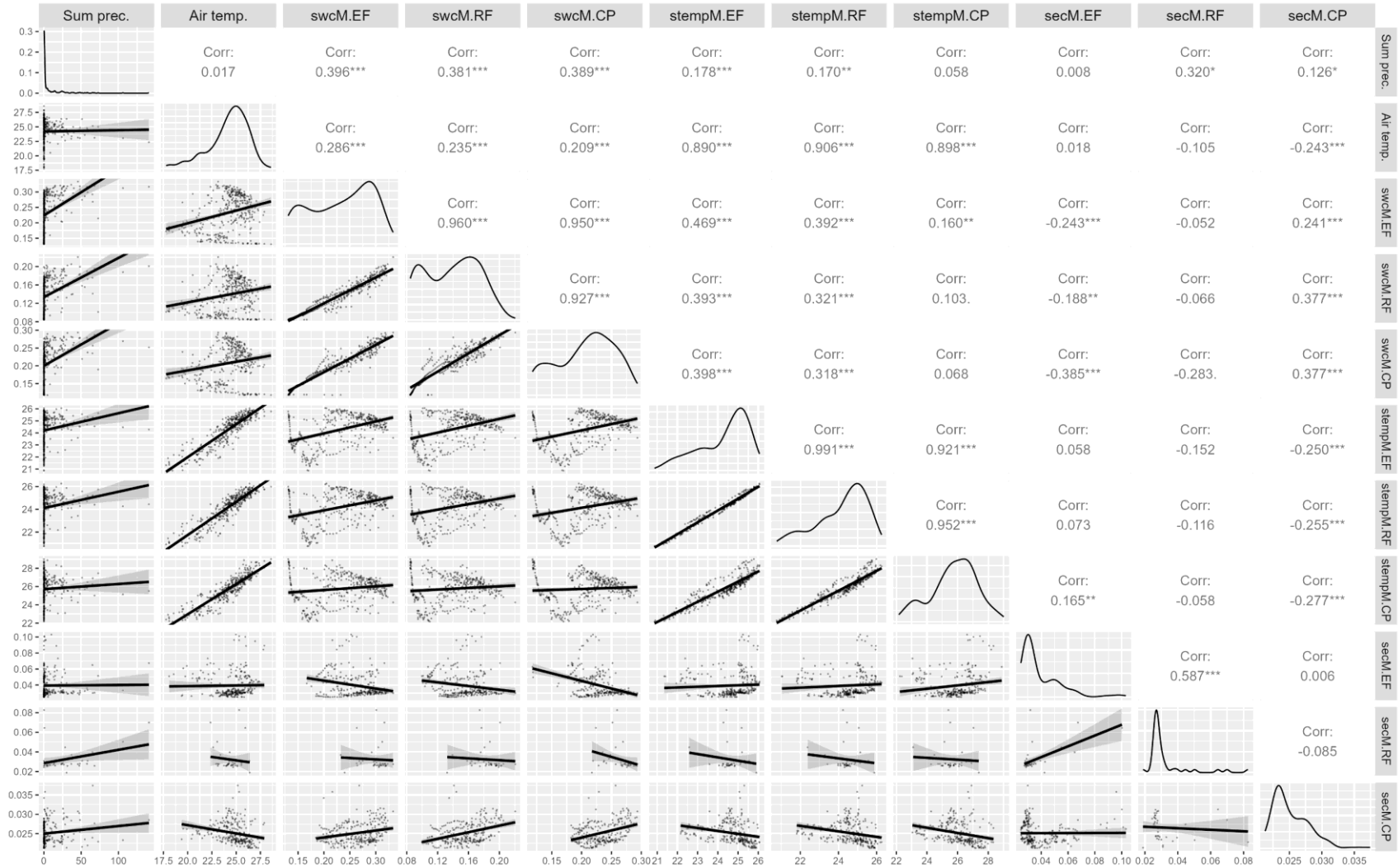
Figure S8. Correlation between daily sum precipitation (‘Sum prec.’; mm), daily mean air temperature (‘Air temp.’; °C), daily mean soil temperatures (‘stemM’; °C), daily mean soil water content (‘swcM’; m 3 m -3 ), daily mean soil saturation extraction electrical conductivity (‘secM’; mS cm -1 ) at Kulen from April 10, 2022, to April 9, 2023. The suffixes ‘EF’, ‘RF’, and ‘CP’ represent evergreen forests, regrowth forests, and cashew plantations. The precipitation and air temperature data were measured at Kulen’s meteorological station (see Fig. 1); meanwhile, the soil data were the average of two measured plots in each land-cover class.
