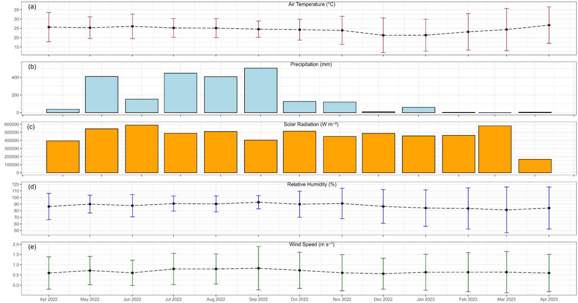
25 Figure S4. Monthly meteorological conditions at Kulen meteorological station from April 10, 2022, to April 9, 2023. (a) Monthly average air temperature (°C); (b) Monthly total precipitation (mm); (c) Monthly total global radiation (W m -2 ); (d) Monthly average relative humidity (%); (e) Monthly average wind speed (m s -1 ). The error bars in (a), (d), and (e) represent the 95% confidence interval (using standard deviation) from the monthly mean. The data were computed based on 15-minute timestep measurements.
