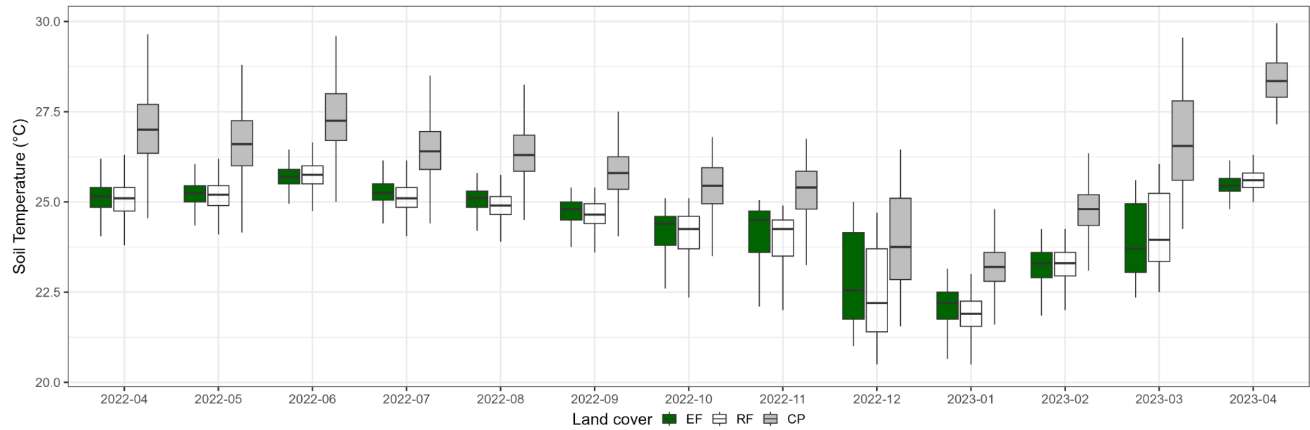
Figure S5. Monthly mean soil temperature (°C) for different land-cover classes from April 10, 2022, to April 9, 2023. The mean values were calculated by averaging the data from two representative plots for each land-cover class. Soil sensors were installed 0.2 m below the ground.
