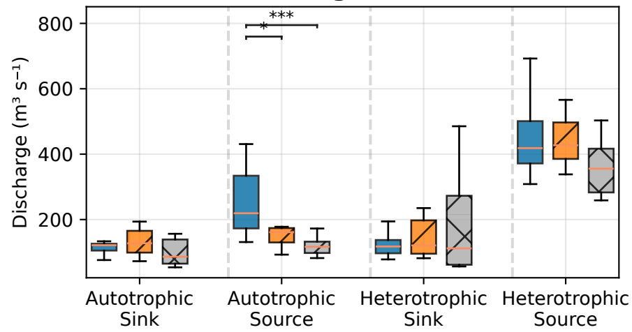
Discharge (m 3 s -1 )
