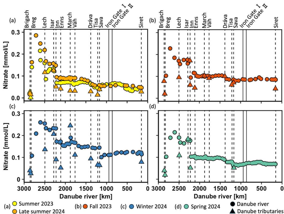
Figure S7: Nitrate concentrations (mmol/L) in the Danube River at various distances from the river mouth. Standard error bars are within the symbol size. Circles represent Danube River samples, triangles denote tributary samples, and dotted lines indicate the river km where tributaries enter. Vertical solid lines represent Iron Gate I and II dams.
