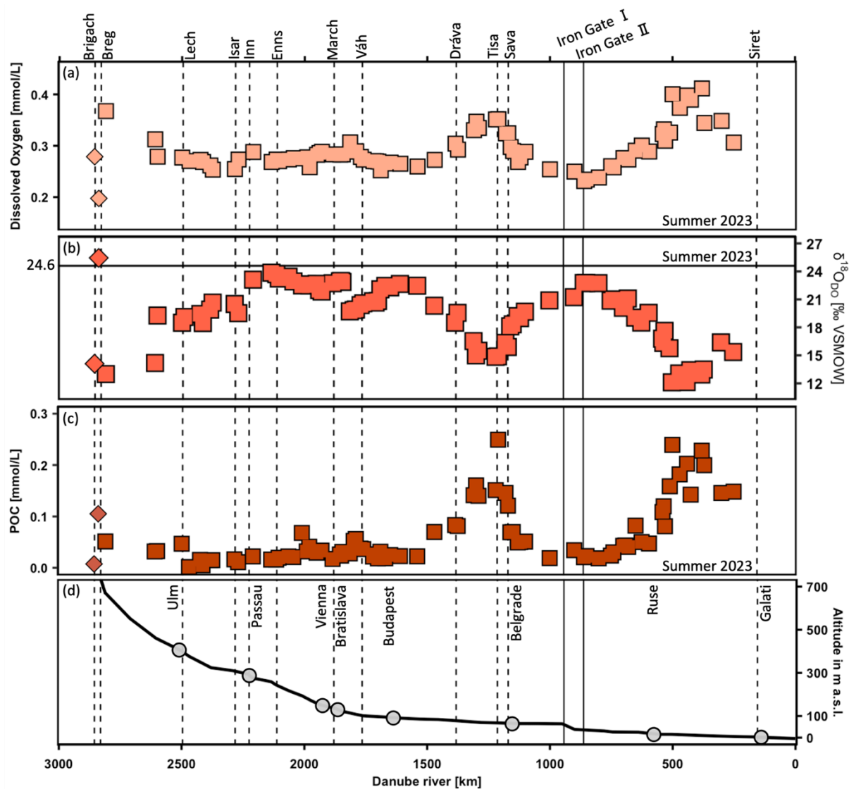
Figure S6: Measurements along the Danube River at various distances from the River mouth during Summer 2023: (a) Dissolved oxygen concentration (mmol/L), (b) Stable isotopes of dissolved oxygen ( \delta^{18}\text{O}_{\text{D}_2\text{O}} ), (c) Particulate organic carbon (POC) concentration (mmol/L) and (d) Altitude (meters above sea level). Squares represent Danube River samples, diamonds indicate tributary samples, and grey dots mark main cities along the river.
