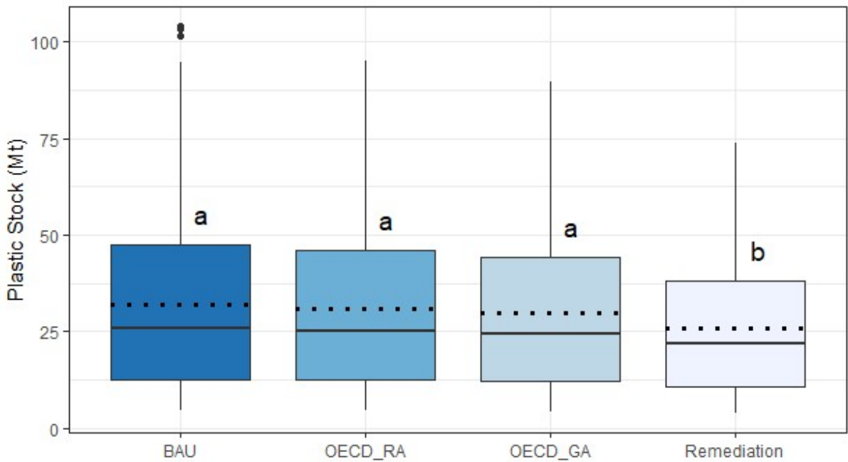
Figure S4: Total marine plastic in 2060 according to the 4 modelled scenarios. Letters indicate significance according to the Dunn post-hoc test. Dotted lines represent the mean, and solid lines the median.
