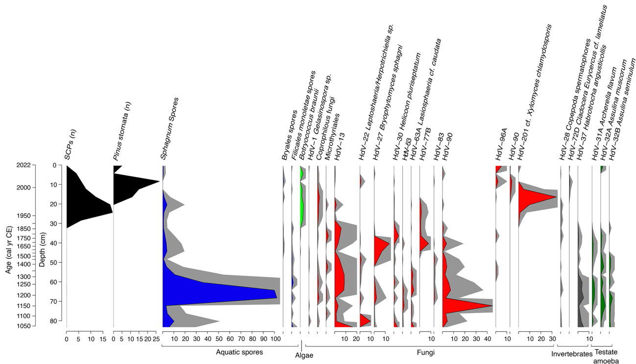
Figure 12. Stratigraphic plot illustrating the abundance of selected non-pollen palynomorphs from core VAR1, as well as spheroidal carbonaceous particles (SCPs) and Pinus stomata , both expressed as counts. Relative abundances of spores of aquatic taxa are shaded blue, algae: light green, fungi: red, invertebrate remains grey and testate amoebae in dark green. Grey shading represents 5× exaggeration. Only taxa with a minimum abundance of 2 % are shown.
