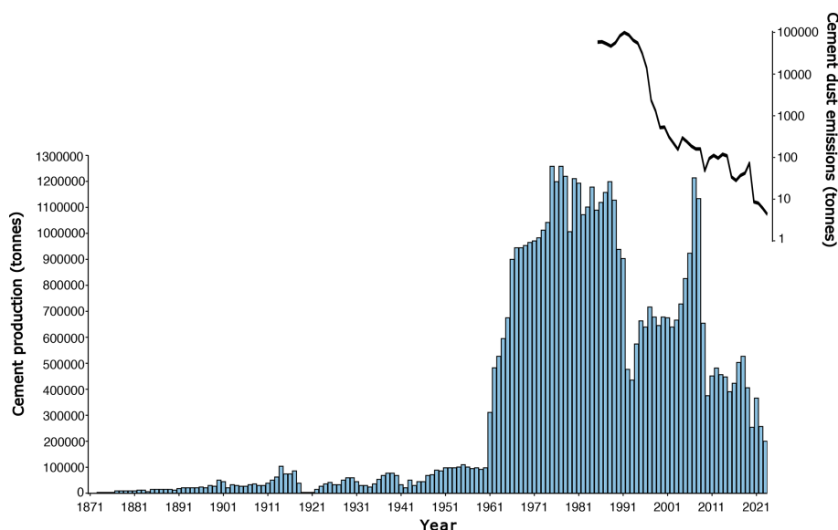
Figure 3. Cement annual production and emissions by the Cement Factory in Kunda. Data adapted from Trumm et al. (2010), digitised from a figure at page 209 using WebPlotDigitiser: https://automeris.io/WebPlotDigitizer/ (last access: 18 November 2024). Emissions data (available from 1985 to 2023) sourced from Raukas (1993); Pärtma (2023) and Heidelberg Materials Kunda AS (2023). Note the logarithmic scale for emission values.
