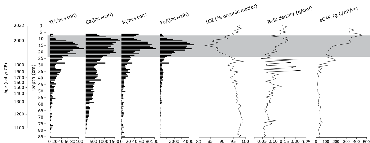
Figure 7. Comparison of selected elements detected by the \mu XRF core scanner, as indicated by the PCA analysis, for the detection of dust fallout from the Kunda cement factory. In addition to peat physical property parameters: Loss on ignition (LOI %), bulk density and apparent carbon accumulation rates (aCAR). \mu XRF Data are presented as counts per second and normalised by dividing the sum of incoherent (inc) and coherent (coh) activities. The shaded area represents the section of core where most of the cement dust is concentrated. The uppermost aCAR sample was removed from the figure to aid interpretation.
