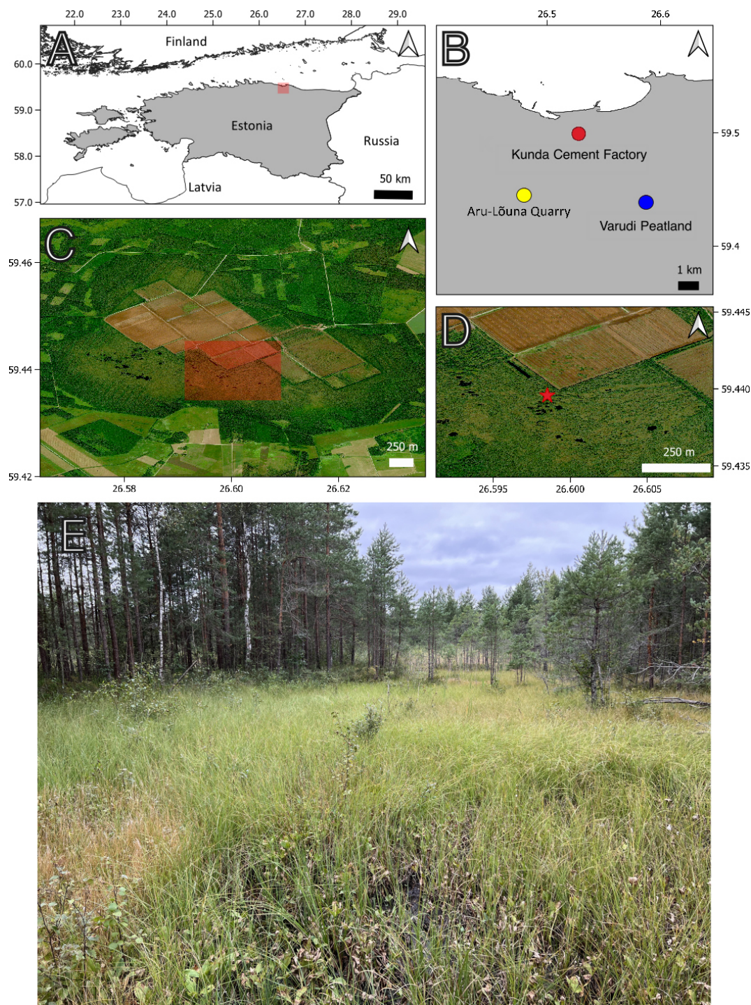
Figure 1. Map of study locations. (A) Modern-day Estonia (in Gray). The red shaded square in map (A) indicates the area mapped in map (B). (B) Locations of sites relevant to this study (Kunda cement factory: Red, Aru-Lõuna Quarry: Yellow, Varudi peatland: Blue). (C) Satellite image of Varudi bog (© Microsoft) showing the extent of peat cutting and drainage that has taken place over the past century. The red shaded area indicates the area mapped in map (D). (D) Close-up of the location from where core VAR1 was recovered (red star). (E) Coring location.
