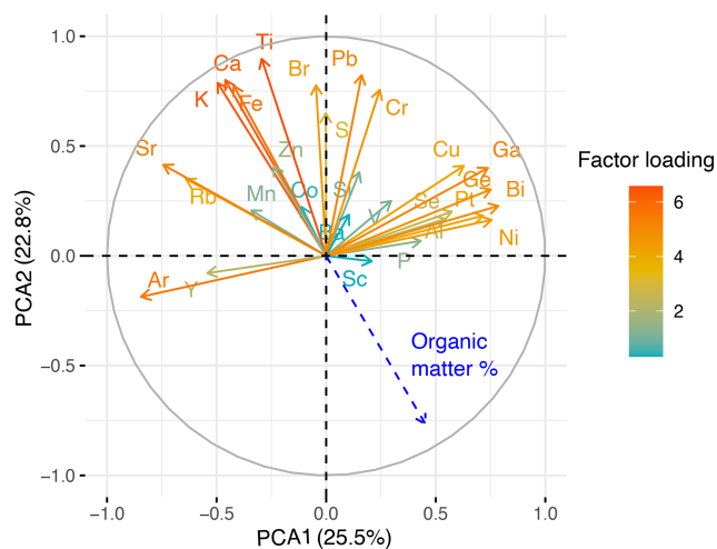
Figure 8. Biplot of first and second principal components showing factor loadings of individual elements scanned across core VAR1. Positively correlated variables point to the same side of the plot, while negatively correlated elements point to the opposite sides. Peat organic matter % (Derived from Loss on Ignition) content is shown in blue. The colour of the lines represents the sum factor loading of each variable for both axes, representing how strongly each variable contributes to the principal component.
