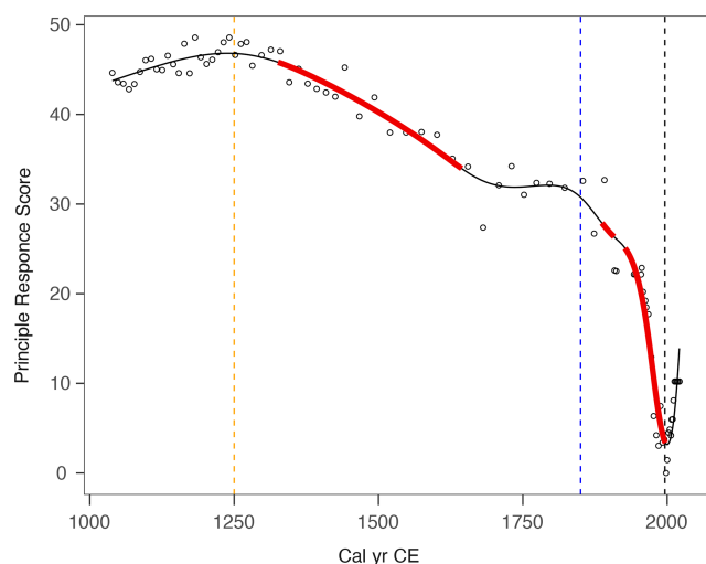
Figure 13. Changes in principal response curve scores derived from sub-fossil testate amoebae data, modelled using an adaptive spline generalised additive model GAM (black line). Solid red lines indicate periods of rapid change, identified where the modelled confidence interval of the slope does not include zero. Vertical dashed lines denote key chronological events potentially influencing environmental conditions at Varudi: The onset of human activity recorded in the pollen data (ca. 1250 cal CE, orange), the beginning of cement production in Kunda (1871, blue) and the installation of pollution control filters at the cement factory (1996, black).
